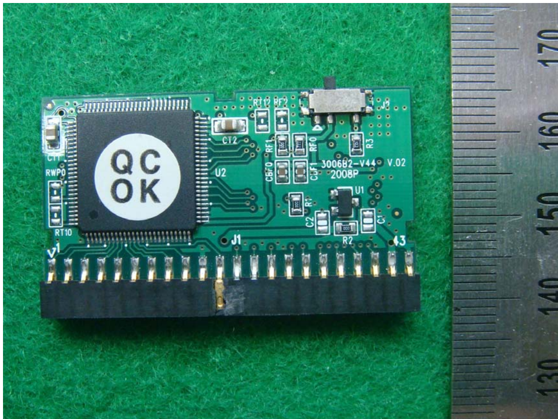
&lt;Photograph 12: SSD Rear view &gt;
