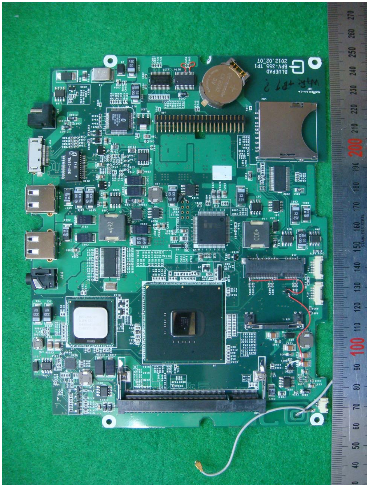
&lt;Photograph 3: Main board Front view(RF module, RAM, SSD removed)&gt;
