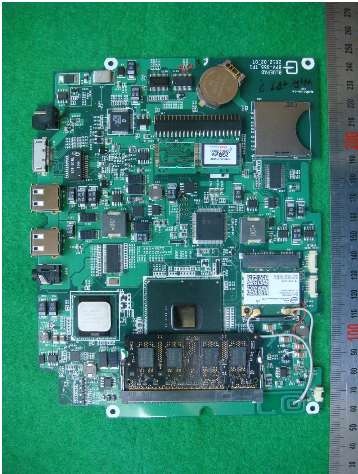
&lt;Photograph 2: Main board- Front view&gt;
