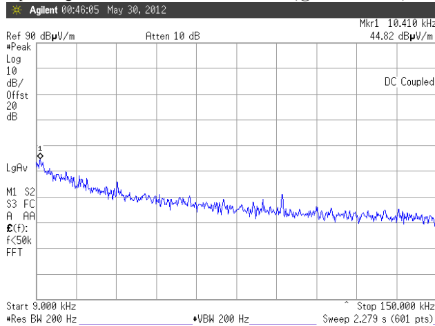
Figure 9. Emission plot for the preliminary radiated measurements
