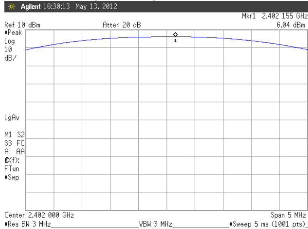
Figure 1. Plot of the Maximum Peak Output Power (Conducted) Basic (GFSK) EDR ( \pi/4 QPSK)
