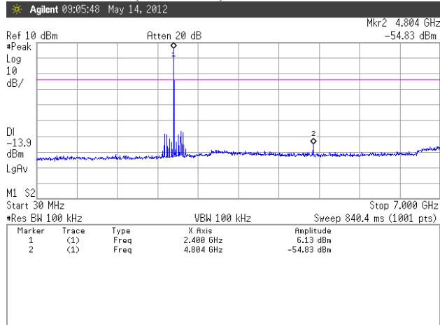
Figure 8. Spurious RF conducted emissions
