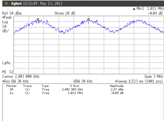
Figure 2. Plot of the Carrier Frequency Separation Basic (GFSK) EDR ( \pi/4 DQPSK)
