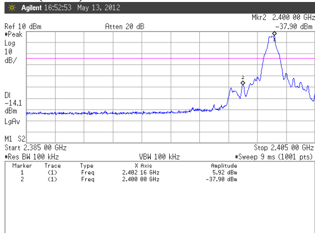
Figure 6. Plot of the Band Edge (Conducted)
