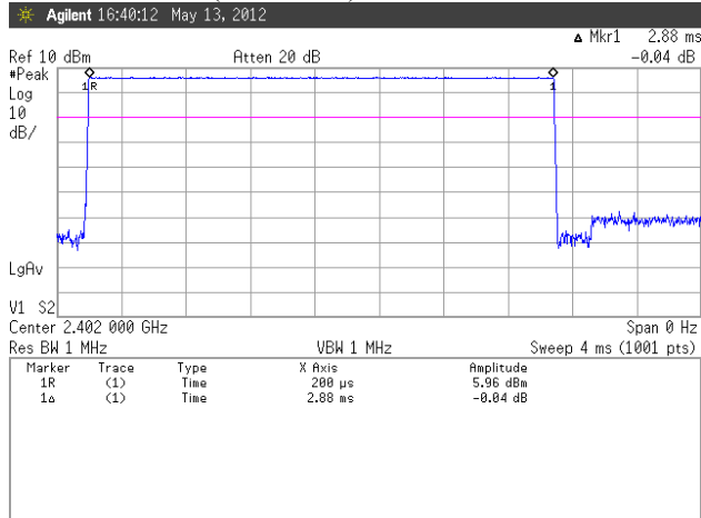
Figure 5. Plot of the Time of Occupancy Basic (GFSK)
