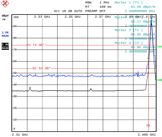
Figure 7. Plot of the Band Edge (Radiated)
