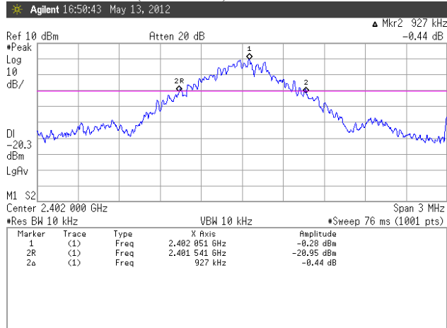
Figure 3. Plot of the 20 dB Channel Bandwidth
