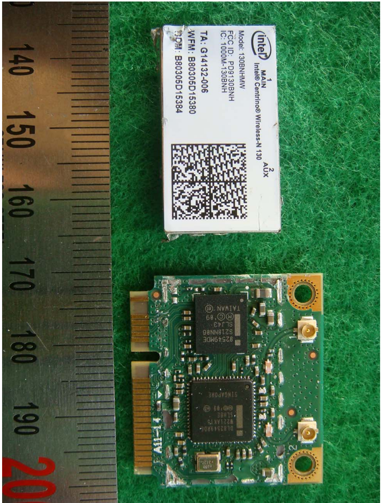
<Photograph 6: WLAN & Bluetooth Module Front view – Label & Shielding removed>
