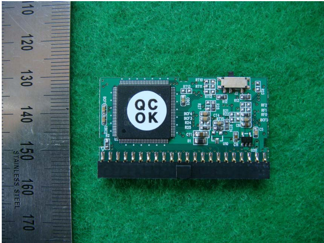
&lt;Photograph 14: SSD Rear view &gt;
