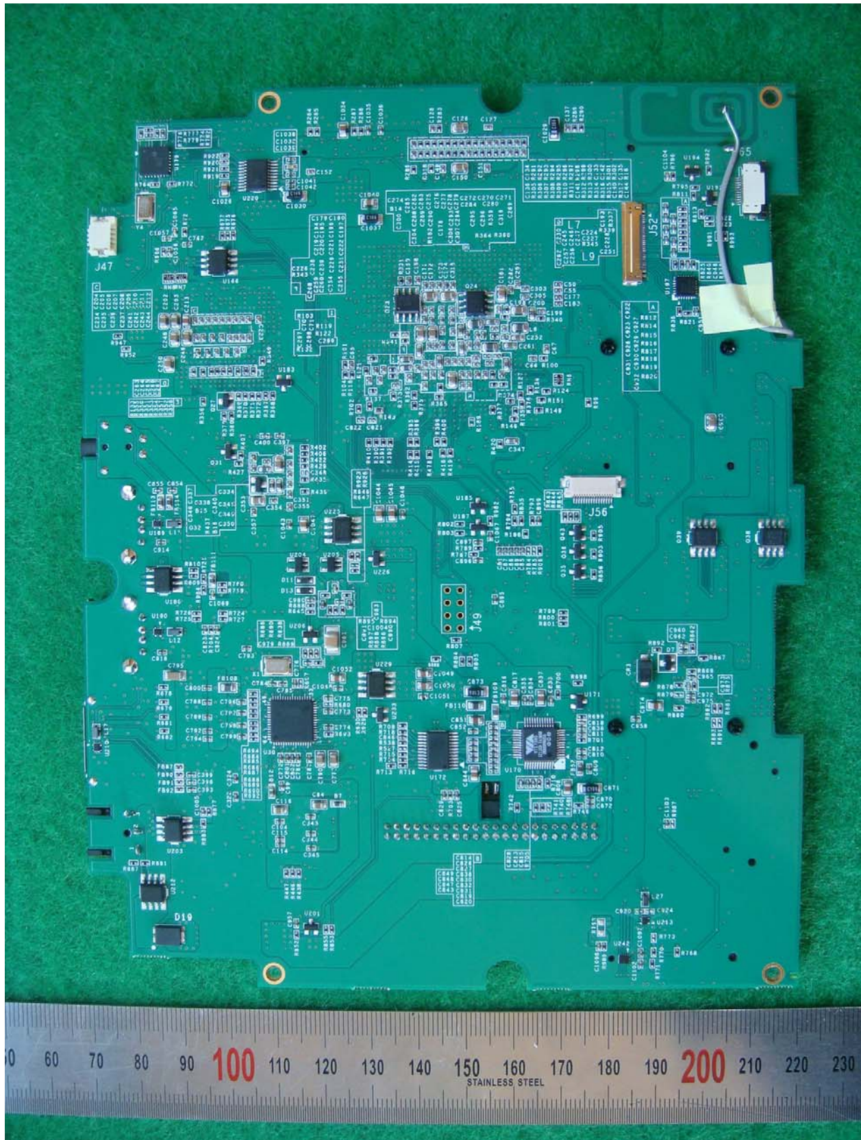
&lt;Photograph 4: Main board Rear view &gt;
