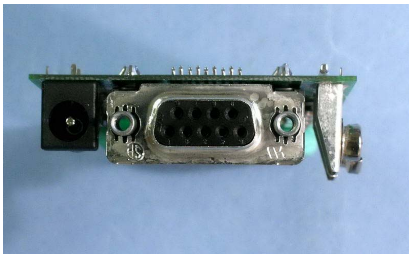
13192-SARD with integrated antenna, view of RS 232 port , AC adapter and DC battery ports
