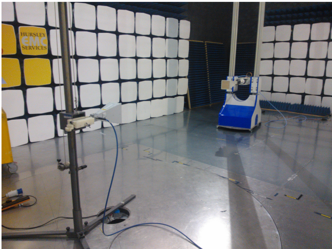
Substitution measurement
