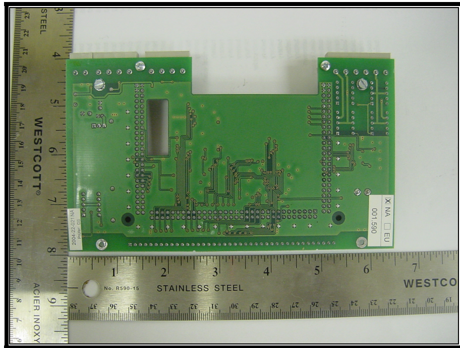
PHOTOGRAPH 24: I/O BOARD BACK
