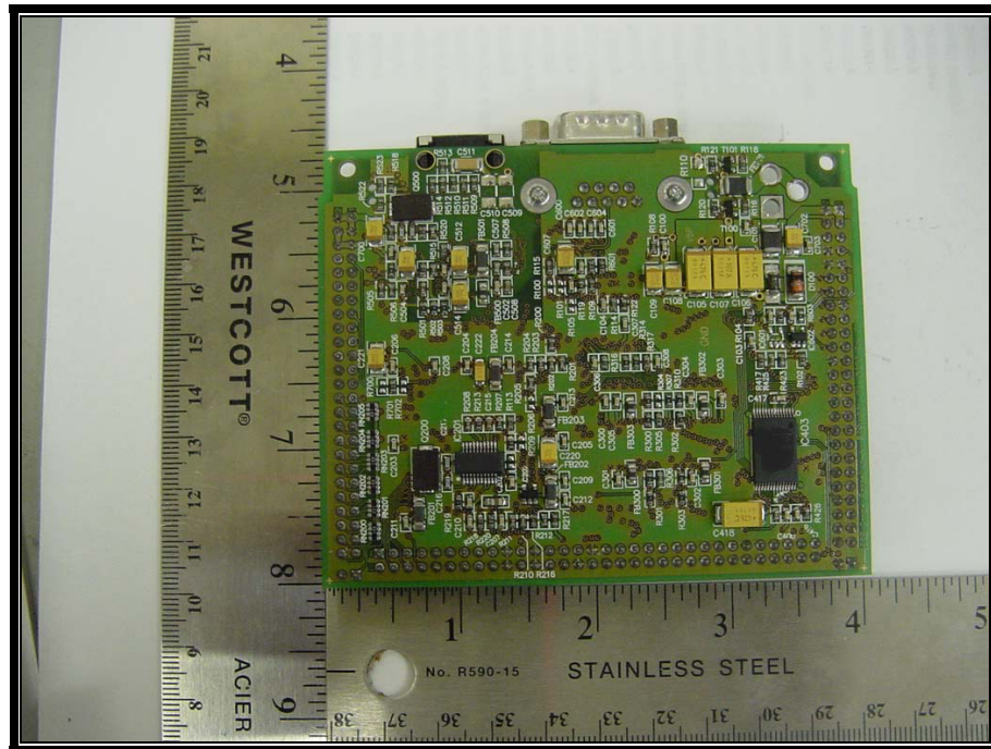
PHOTOGRAPH 20: CPU BOARD BACK
