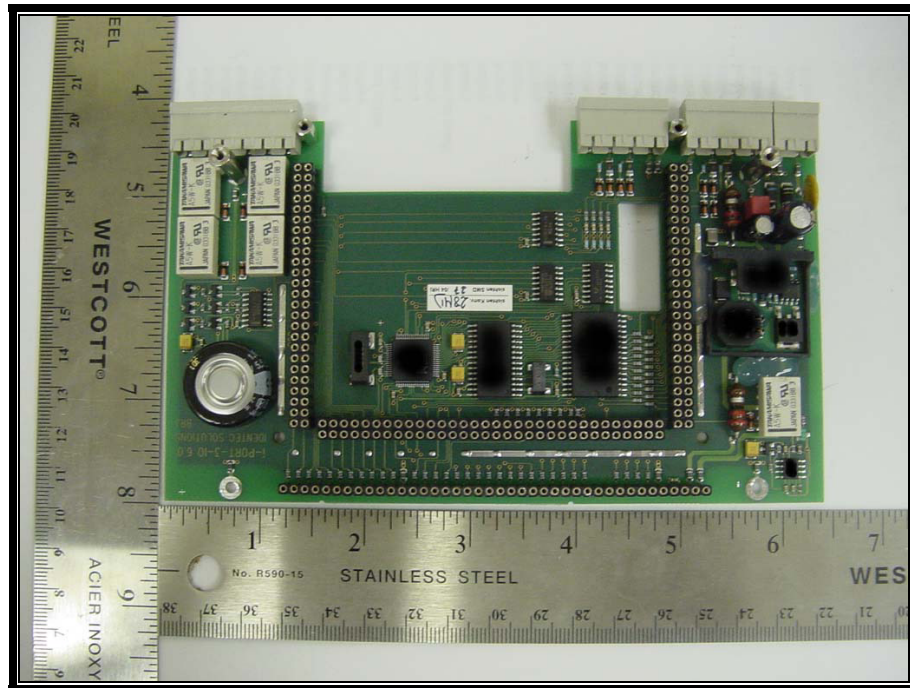
PHOTOGRAPH 23: I/O BOARD FRONT
