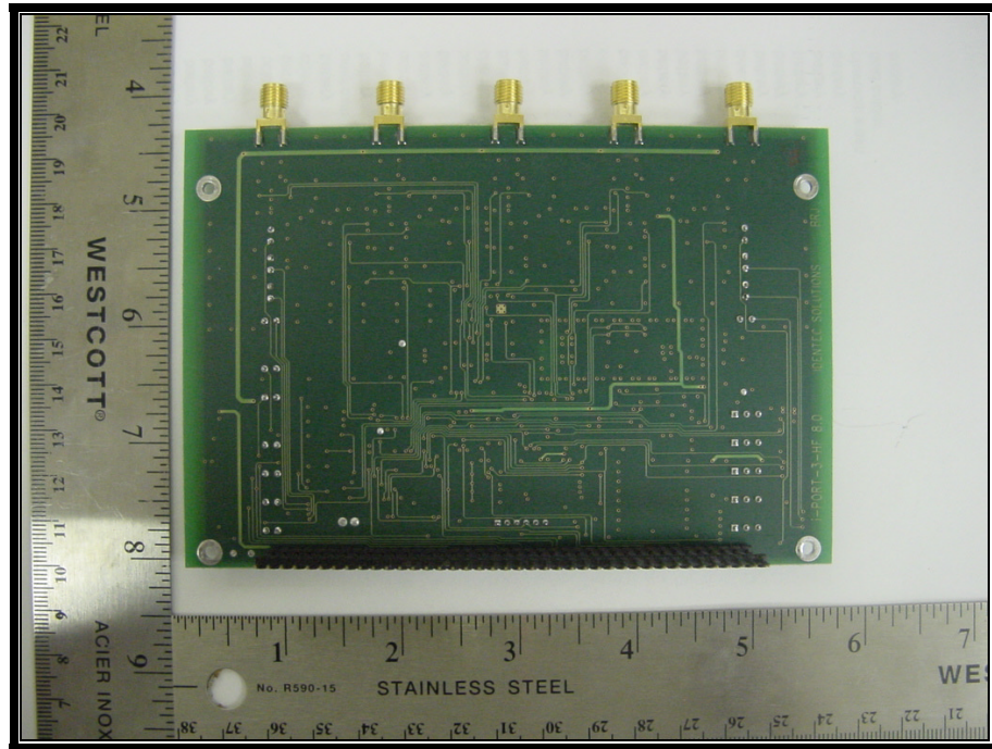
PHOTOGRAPH 22: RF BOARD BACK
