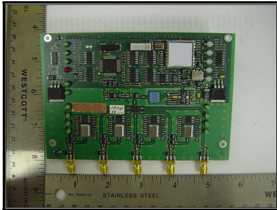
PHOTOGRAPH 21: RF BOARD FRONT
