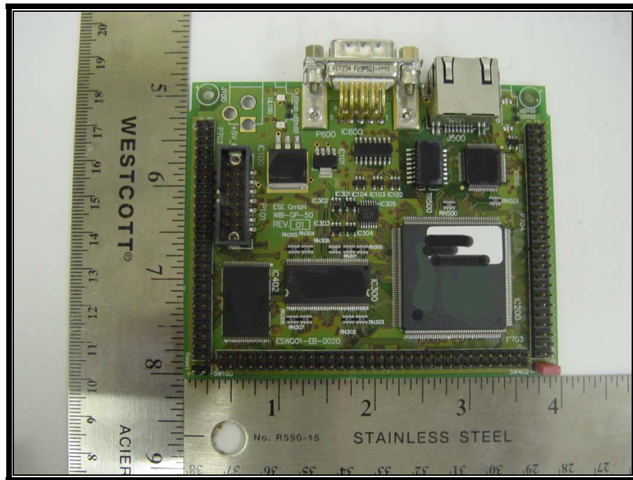
PHOTOGRAPH 19: CPU BOARD FRONT
