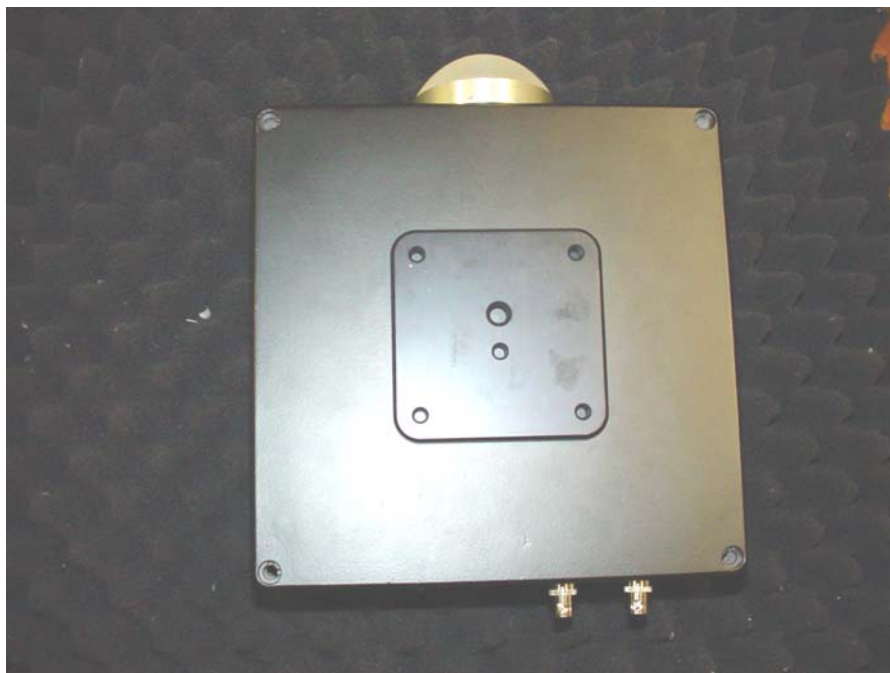
TX Module bottom view showing tripod mounting plate
