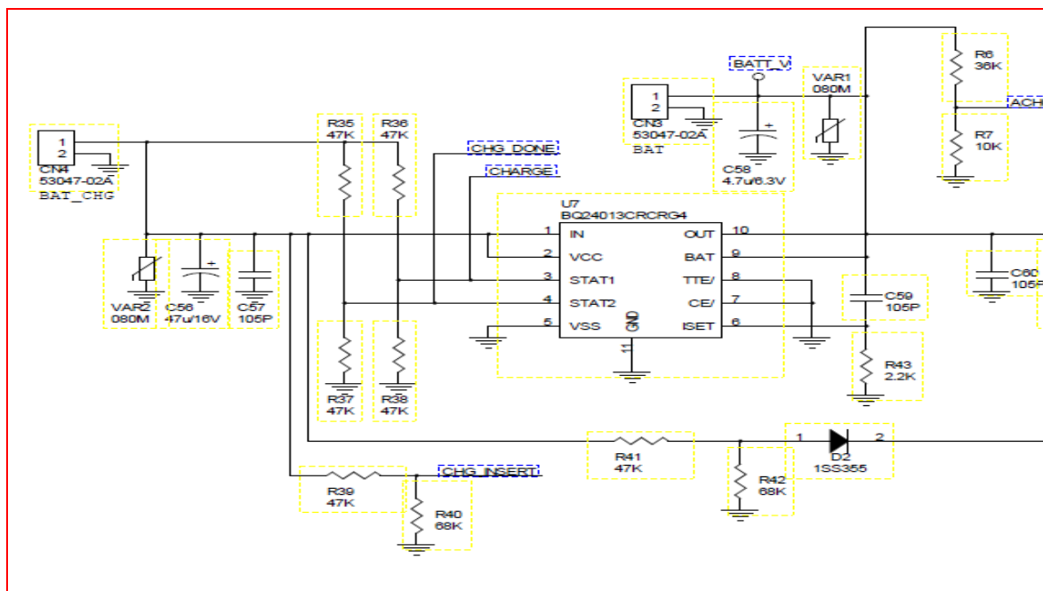
6-8 Battery charger circuit
