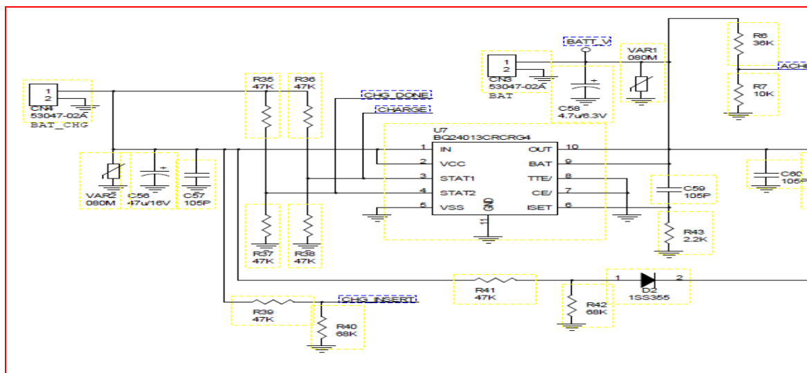
6-8 Battery charger circuit
