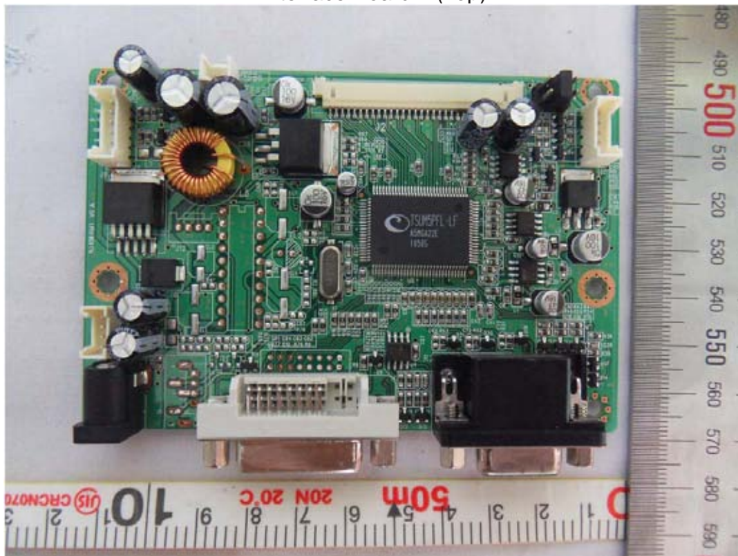
Interface Board 1 (Top)
