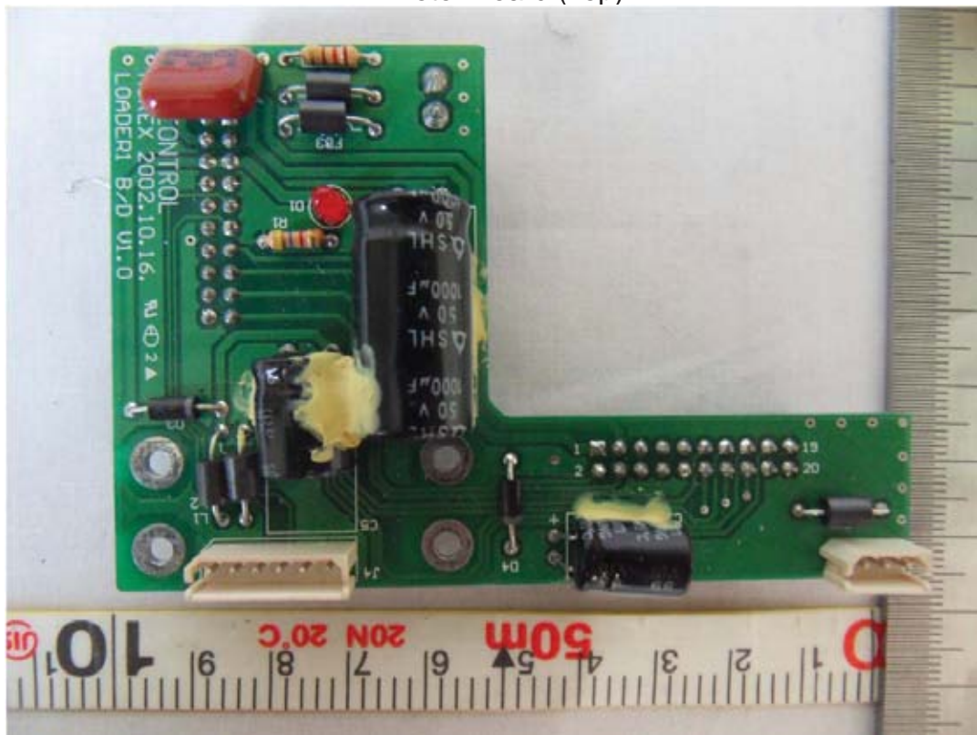
X Motor Board (Top)
