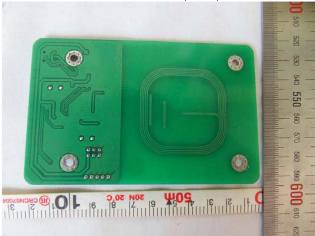
RFID Reader Board (Bottom)
