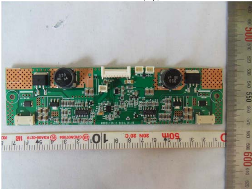
Control Board (Top)
