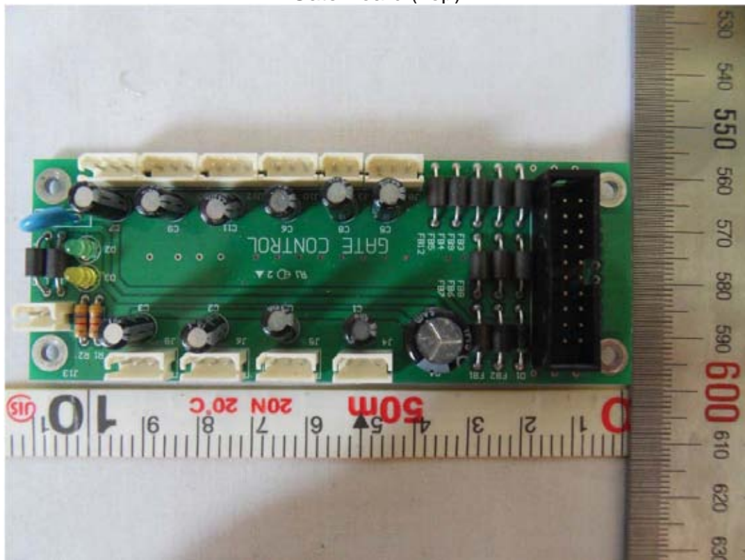
Gate Board (Top)
