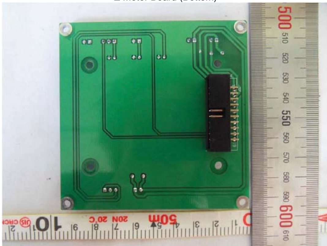
Z Motor Board (Bottom)
