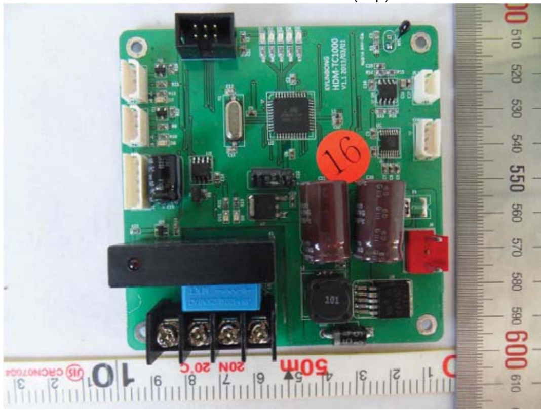
Heater/FAN Control Board (Top)
