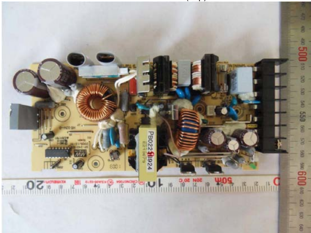
SMPS Main Board (Top)
