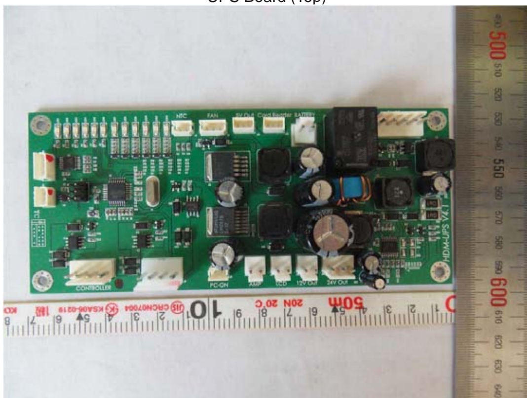
UPS Board (Top)
