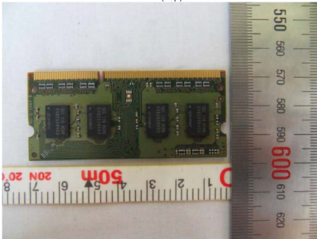
RAM (Top)
