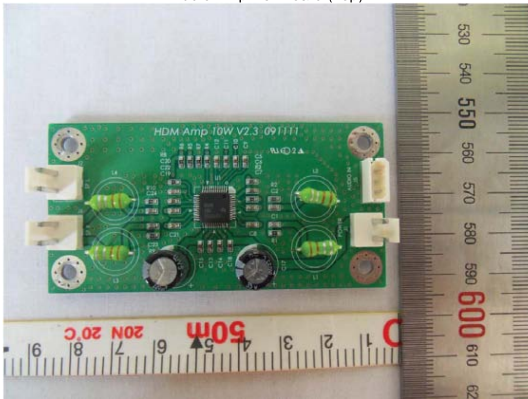
Audio Amplifier Board (Top)
