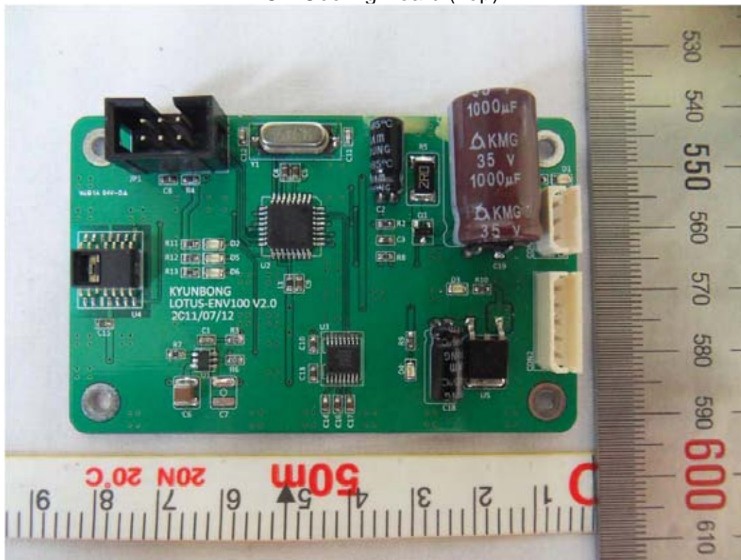
LCD Cooling Board (Top)
