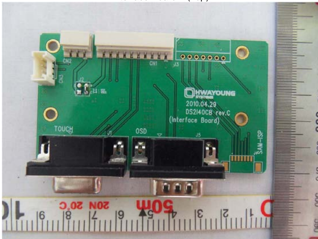
Interface Board 2 (Top)
