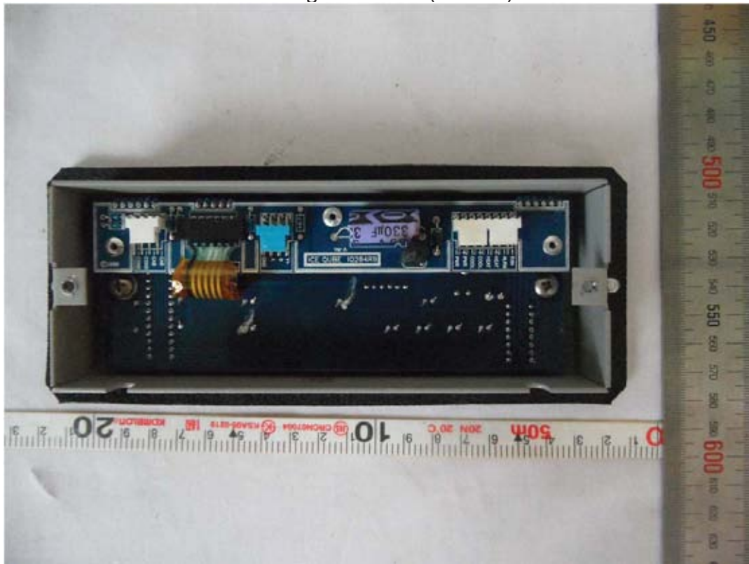
Cooling Controller (Bottom)
