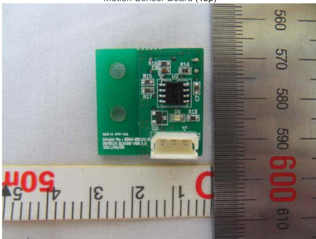
Motion Sensor Board (Top)
