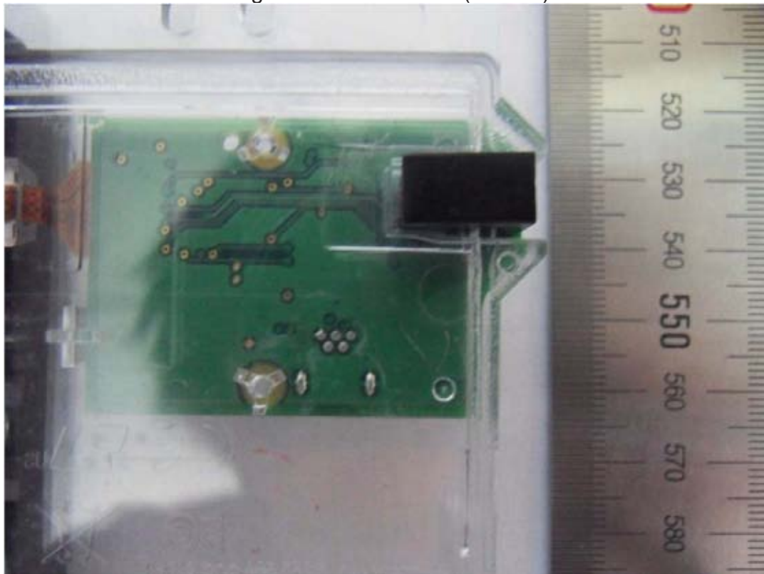
Magnetic Leader Board (Bottom)
