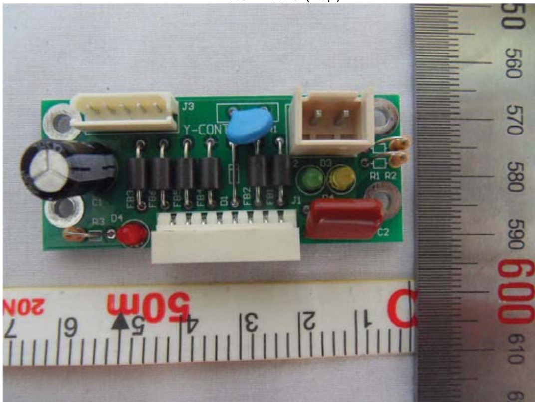
Y motor Board (Top)
