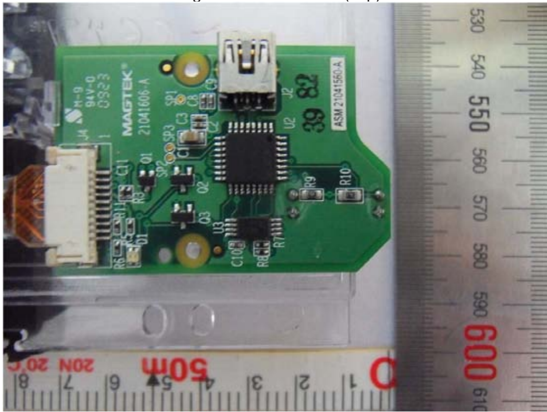
Magnetic Leader Board (Top)
