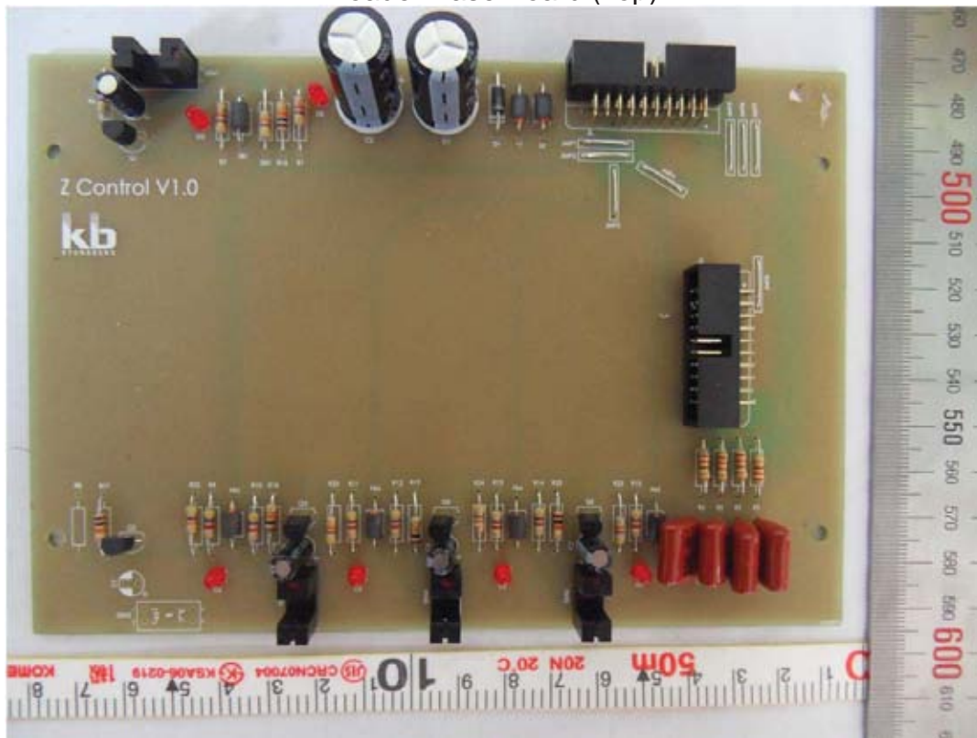
Loader Base Board (Top)
