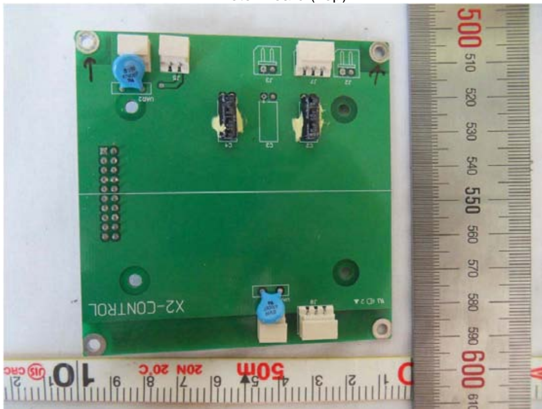
Z Motor Board (Top)
