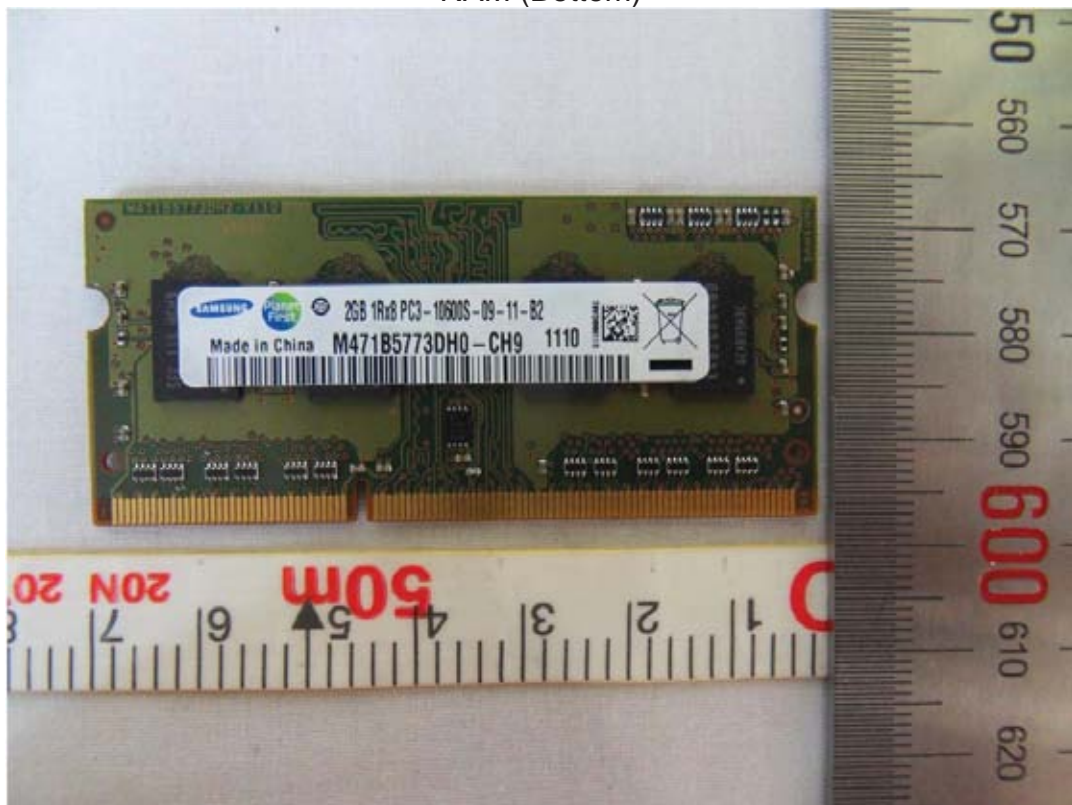
RAM (Bottom)
