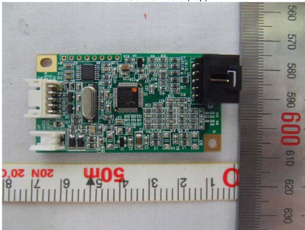
Touch Control Board (Top)
