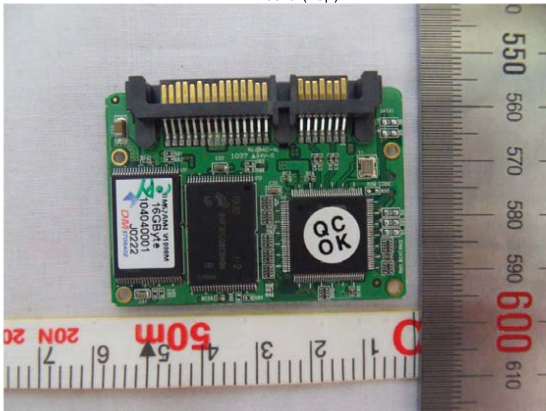
HDD Board (Top)
