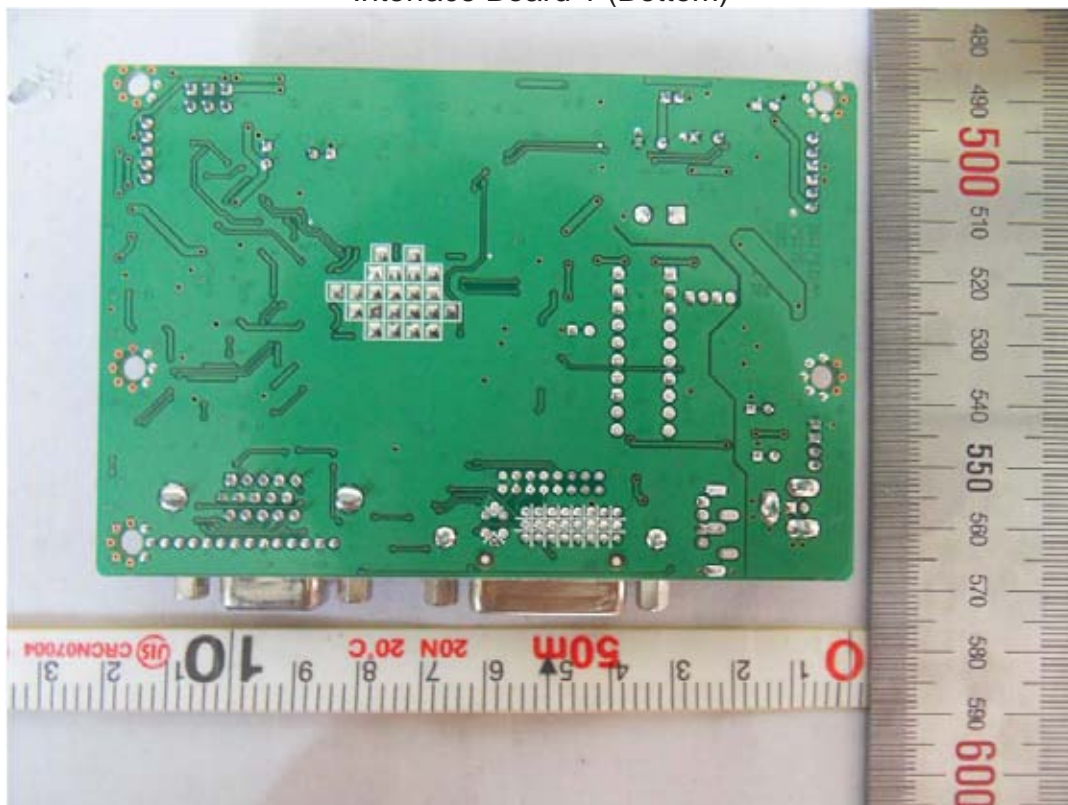
Interface Board 1 (Bottom)
