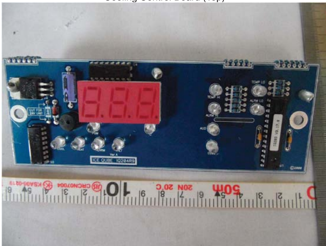
Cooling Control Board (Top)
