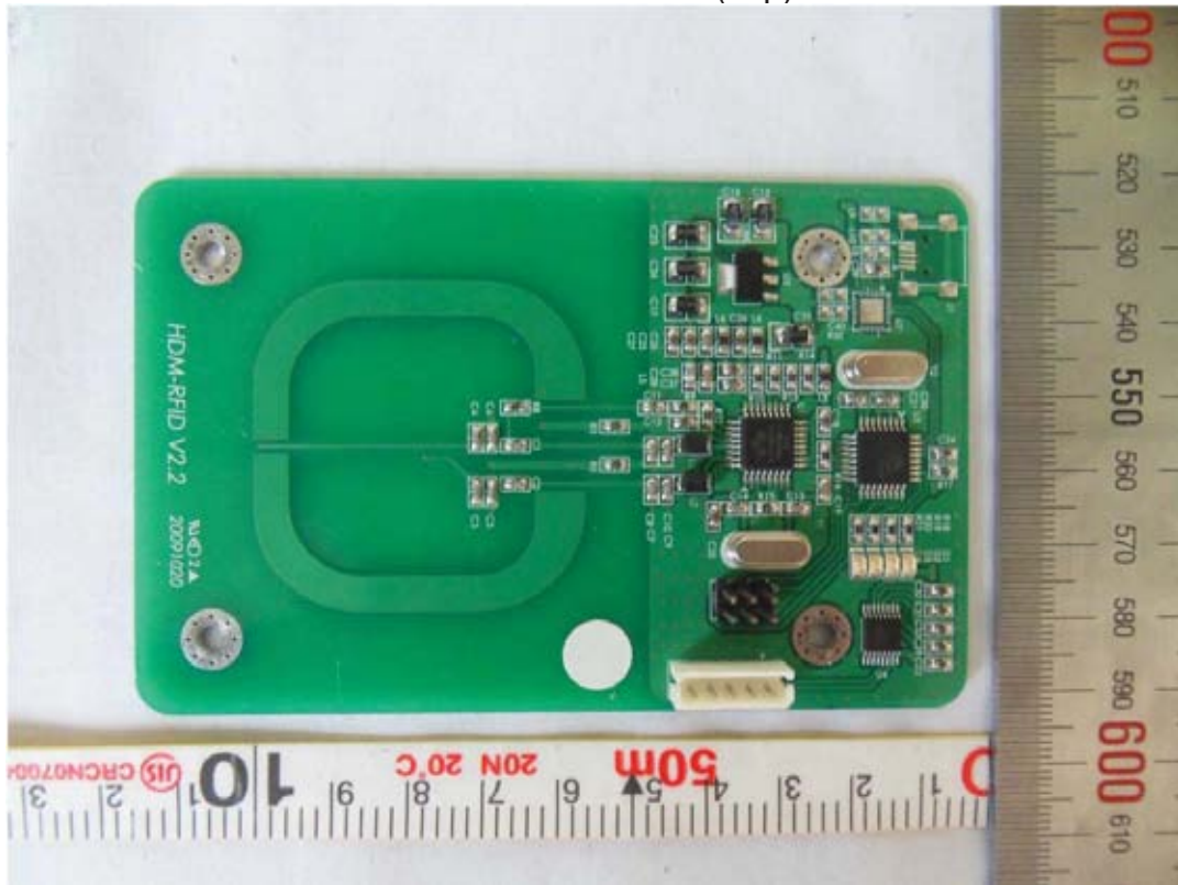
RFID Reader Board (Top)
