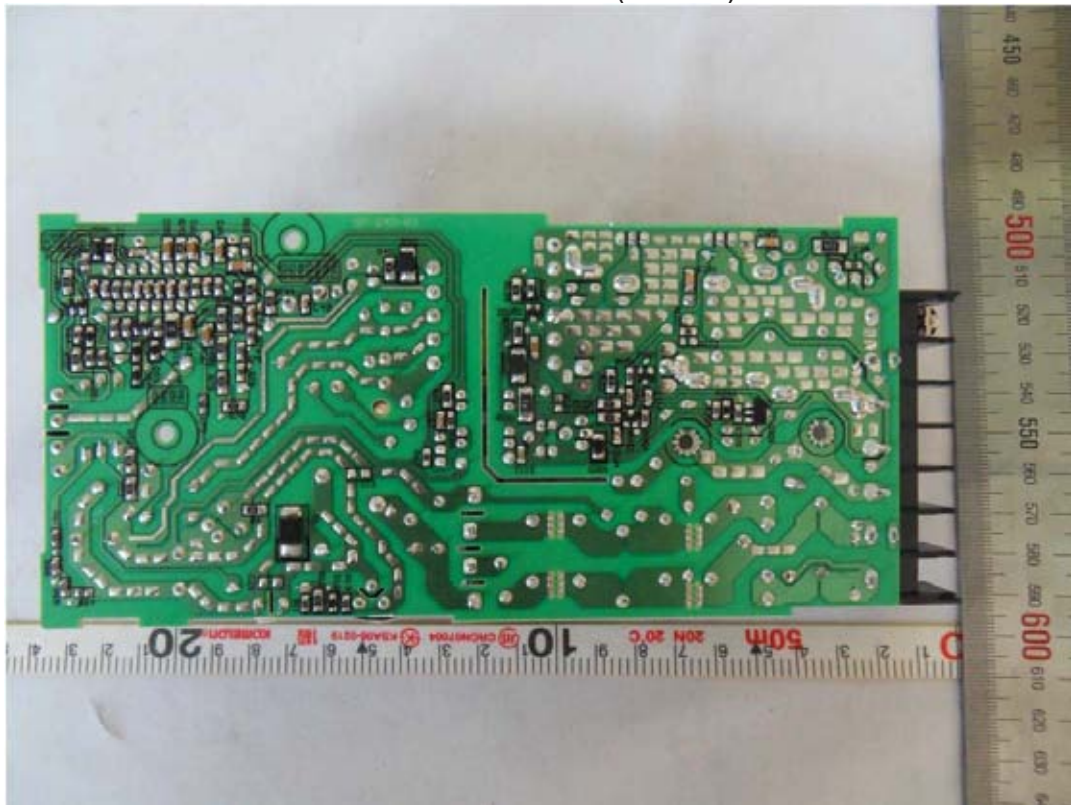
SMPS Main Board (Bottom)
