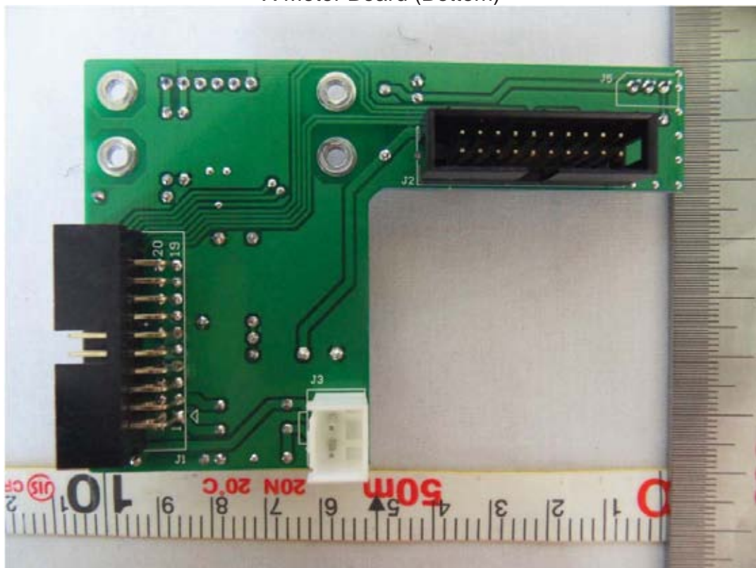
X Motor Board (Bottom)
