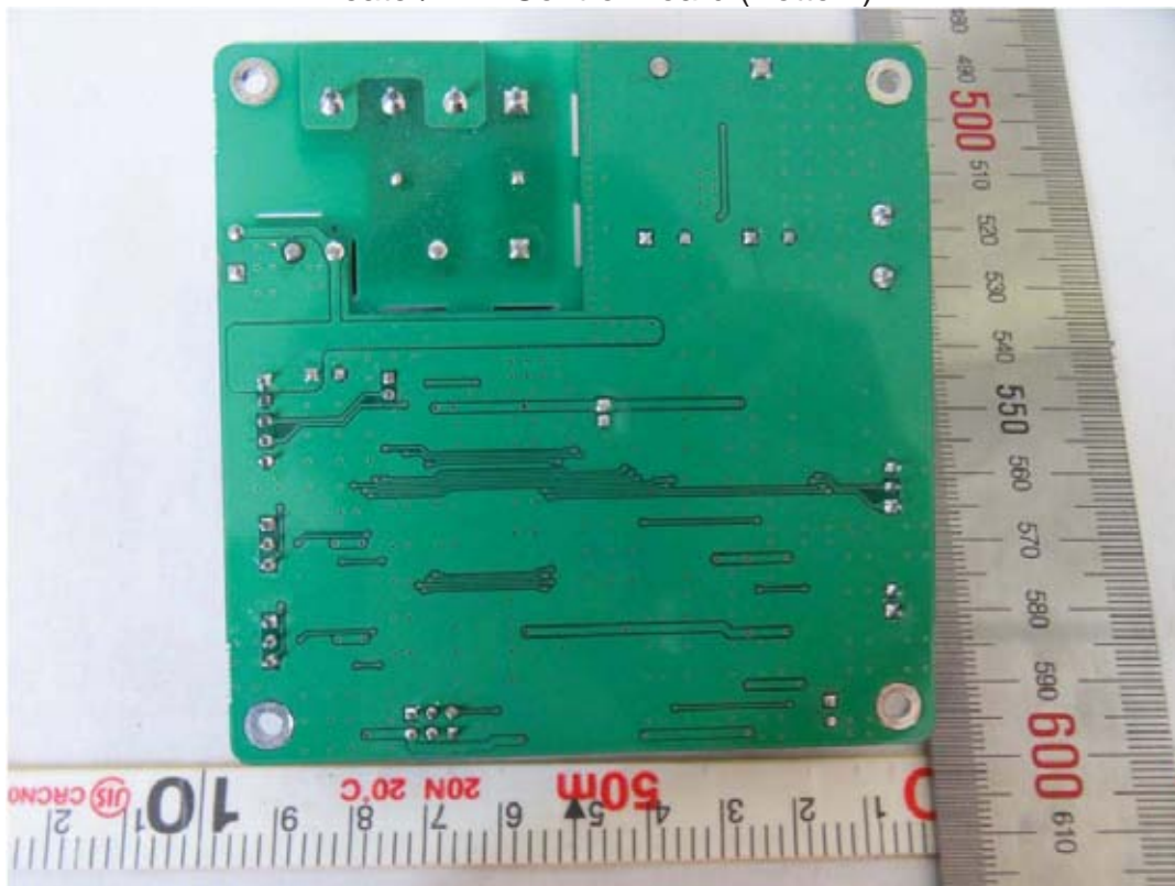
Heater/FAN Control Board (Bottom)
