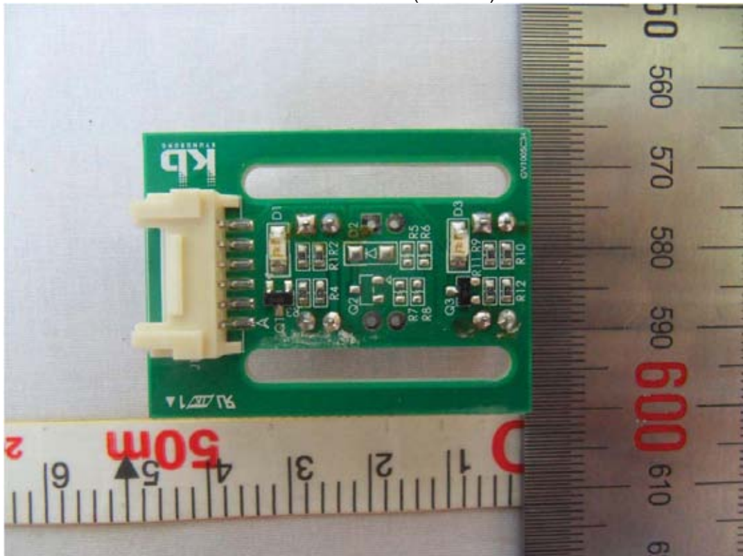
Sensor Board 2 (Bottom)
