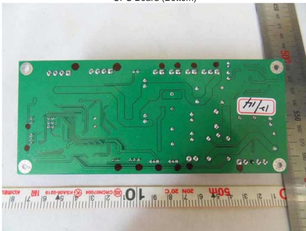
UPS Board (Bottom)
