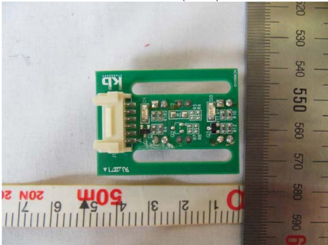
Sensor Board 1 (Bottom)
