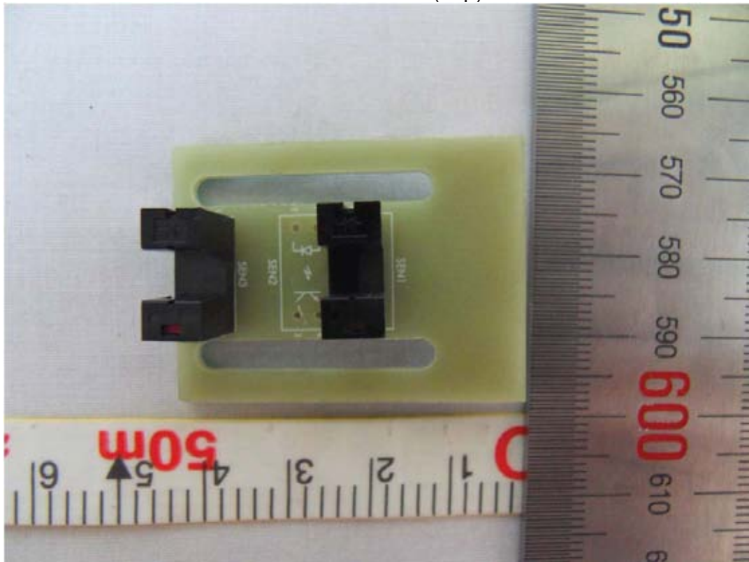
Sensor Board 2 (Top)
