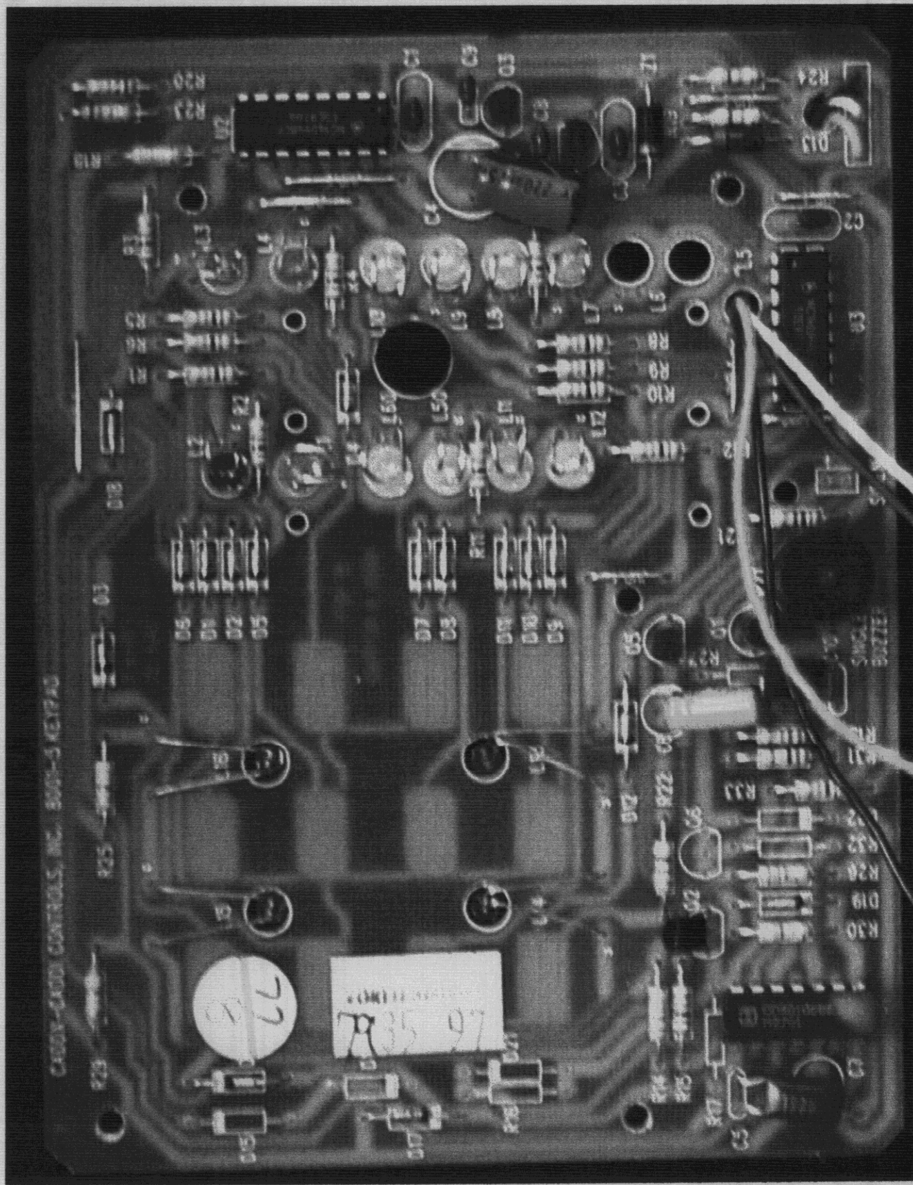
Photo 16. Top View of Button Interface Board
