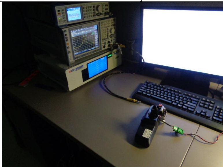
Conducted Setup
