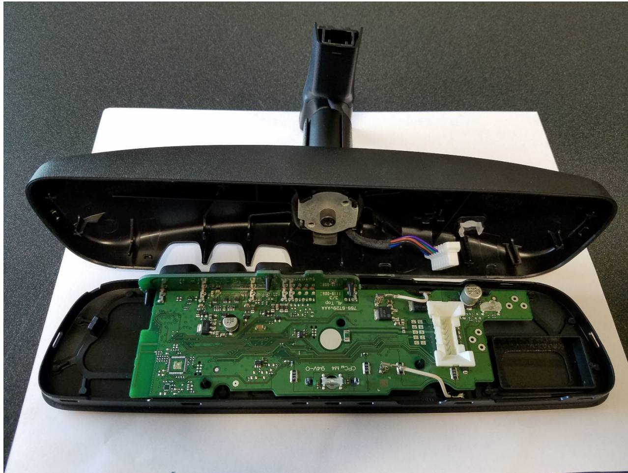
UAHL5F – Internal Photos
