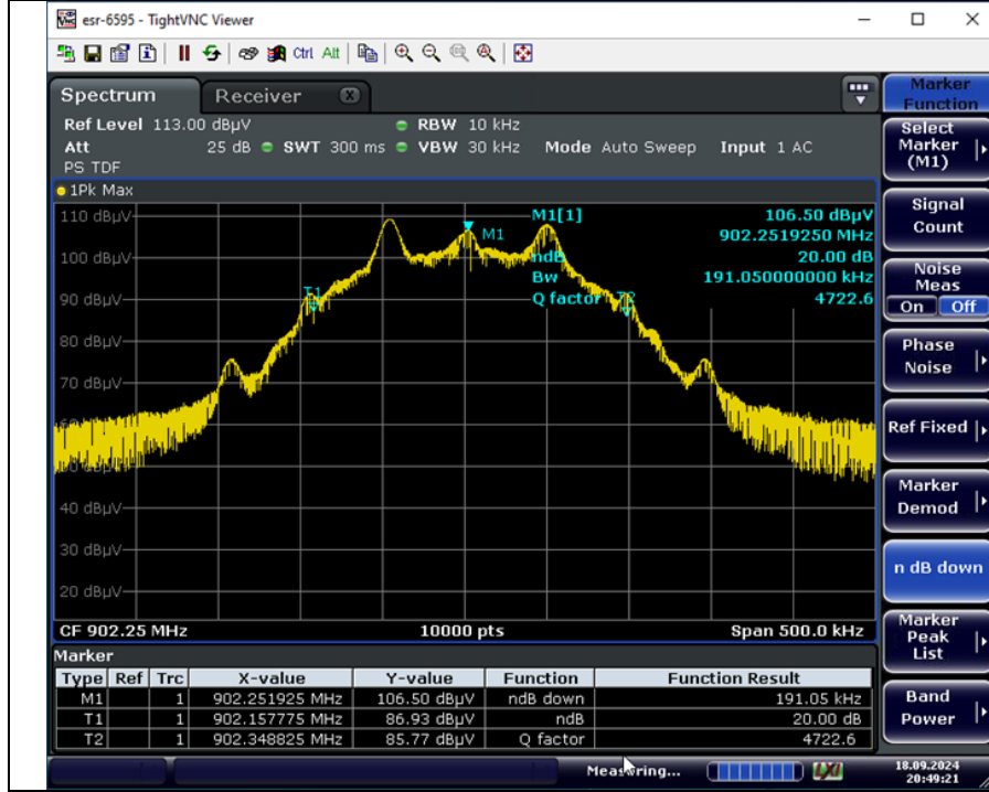
20 dB BW Low Band Measurement Plot
