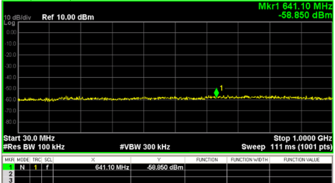
Channel 78; (30~1000) MHz
