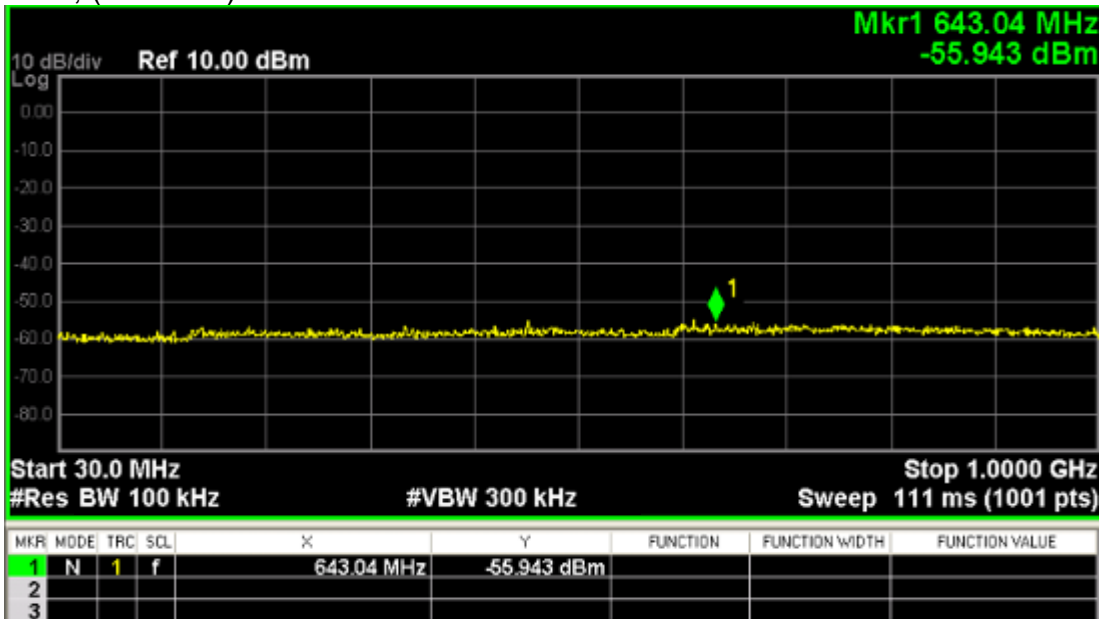
Channel 39; (30~1000) MHz
