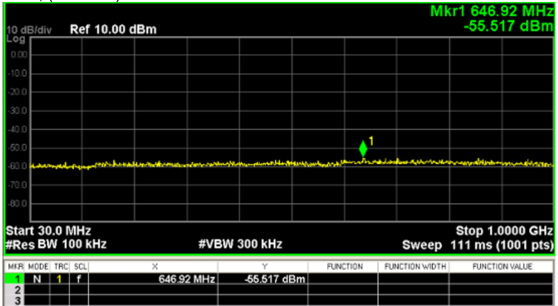
Channel 78; (30~1000) MHz
