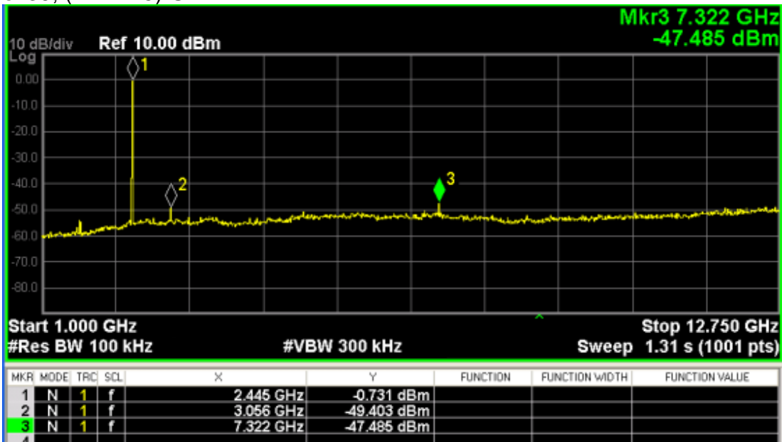
Channel 39; (1~12.75) GHz
