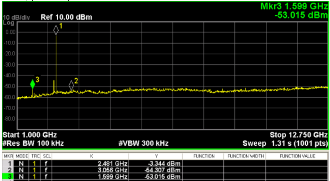
Channel 78; (1~12.75) GHz
