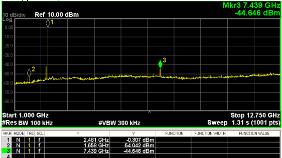
Channel 78; (1~12.75) GHz
