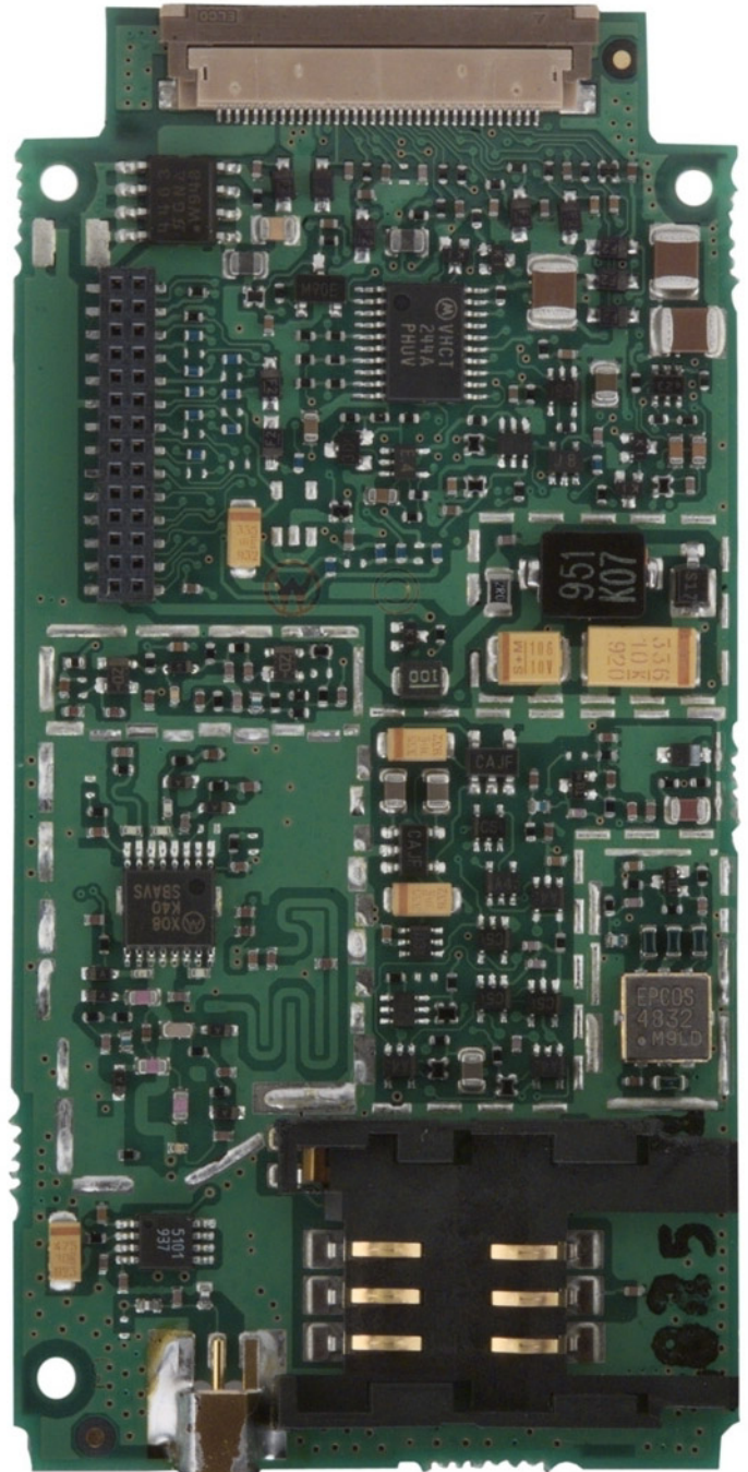
Typical Unit (Top View Shields Removed)
