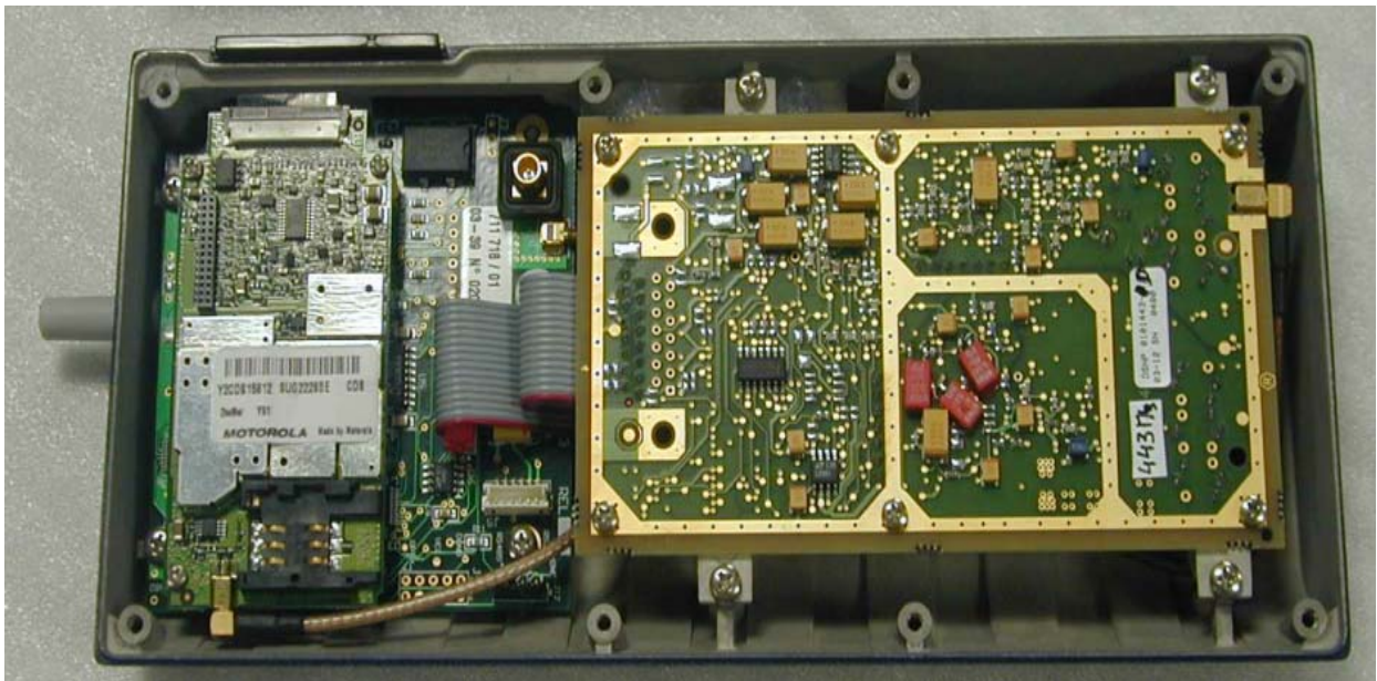
GSM module and Thales Receiver installed in the Com Module
