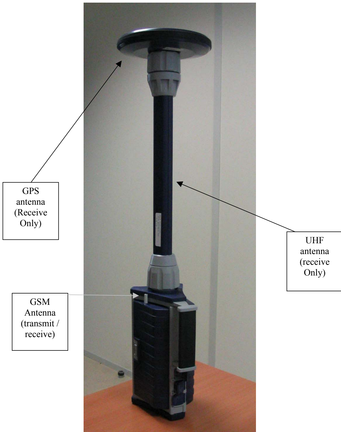
Side View of The System – GPS antenna and UHF antenna
