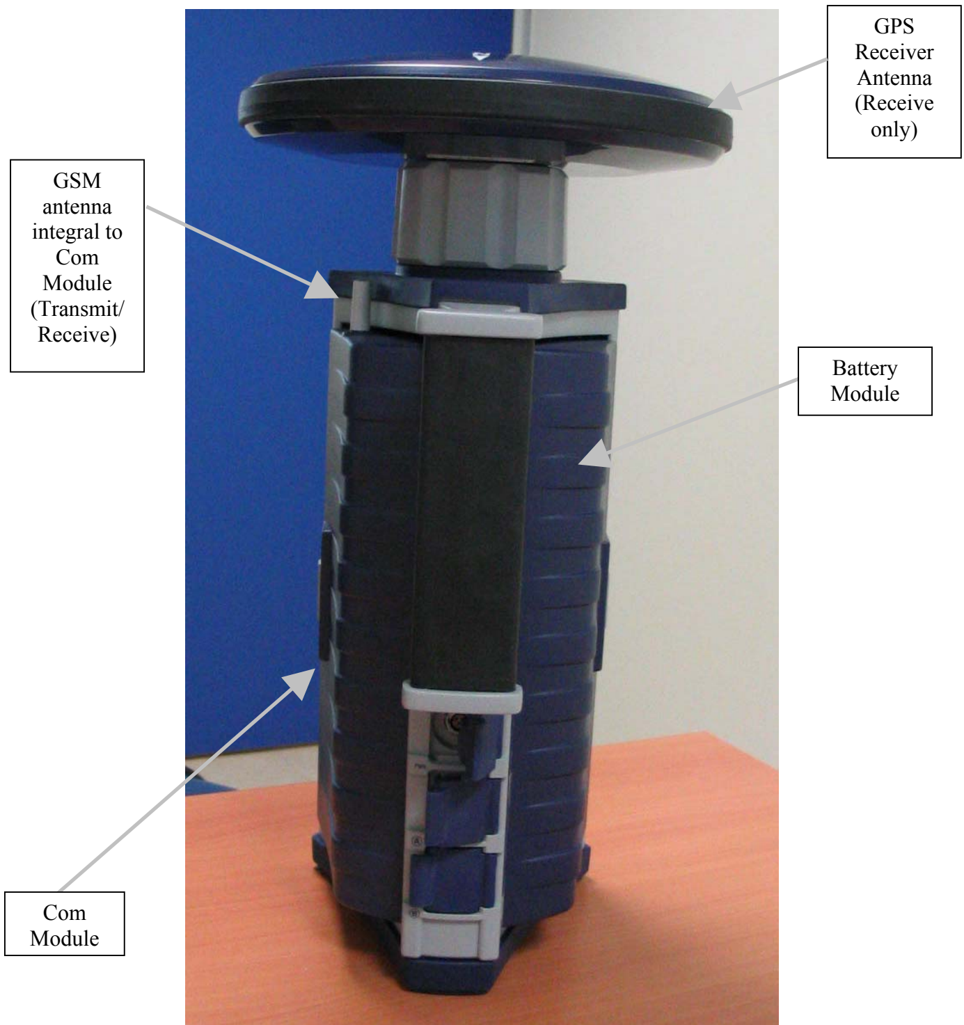
Rear View of The System – GPS antenna but no UHF antenna
