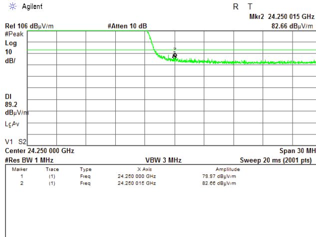
Plot 7.4.4 High band edge emission test result
