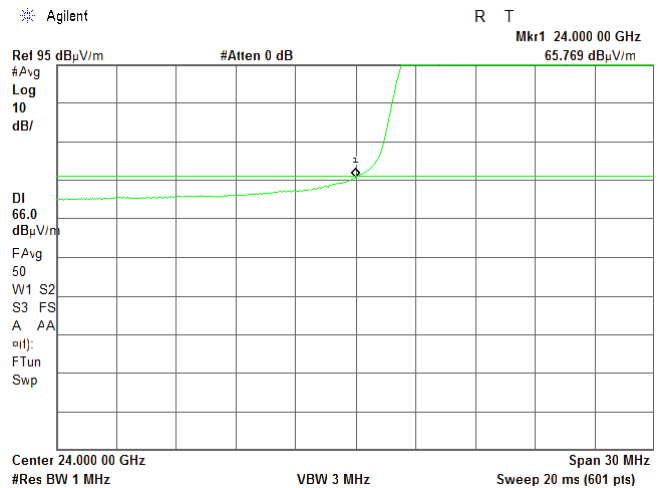
Plot 7.5.6 Low band edge emission test result
