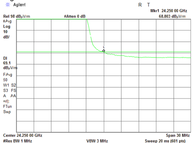
Plot 7.5.4 High band edge emission test result
