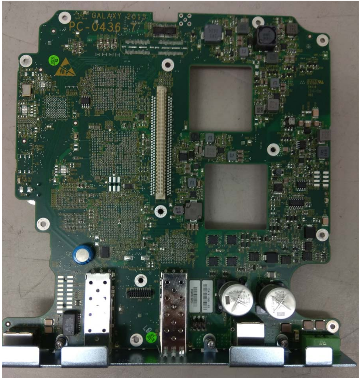
Photograph No.5 “FibeAir IP-20S 24” main board front view
