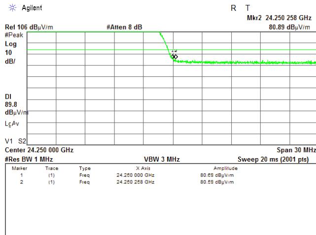
Plot 7.5.6 High band edge emission test result
