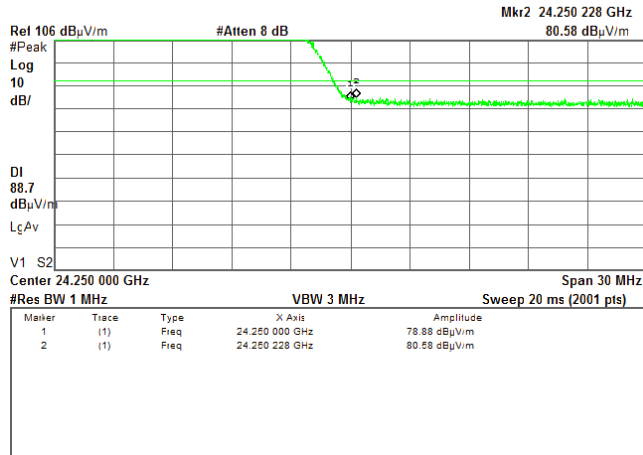
Plot 7.5.16 High band edge emission test result
