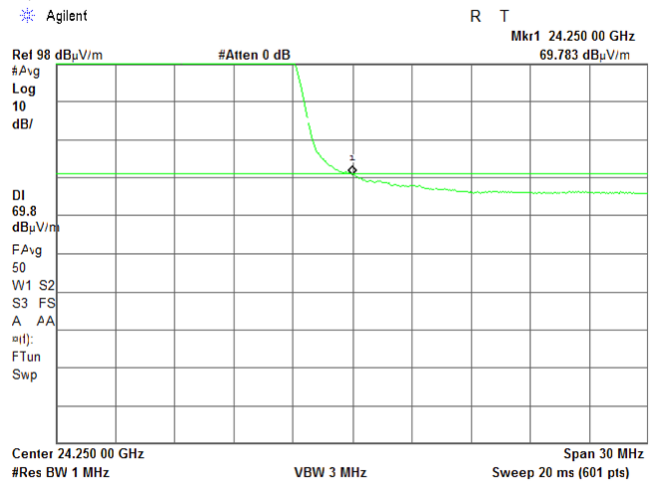
Plot 7.5.6 High band edge emission test result
