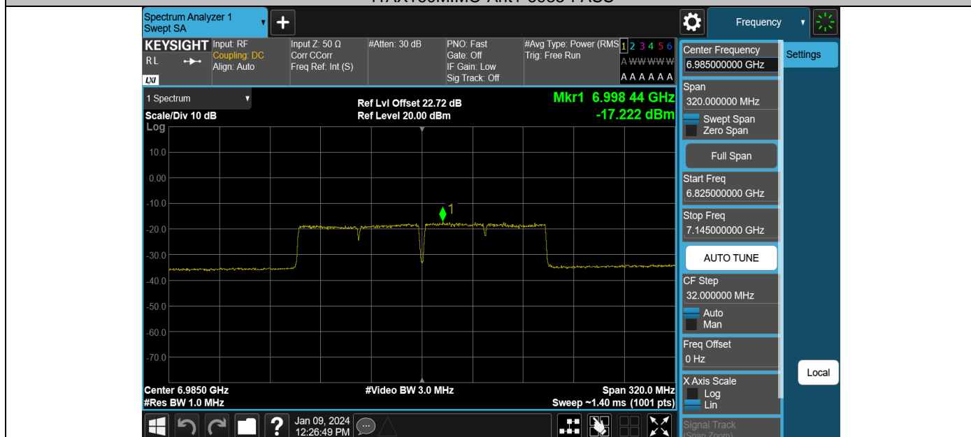
11AX160MIMO-Ant2-6985-PASS
