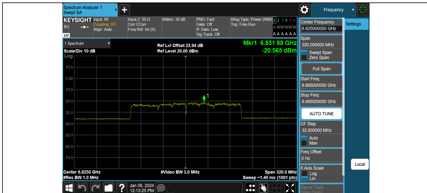
11AX160MIMO-Ant2-6825-PASS
