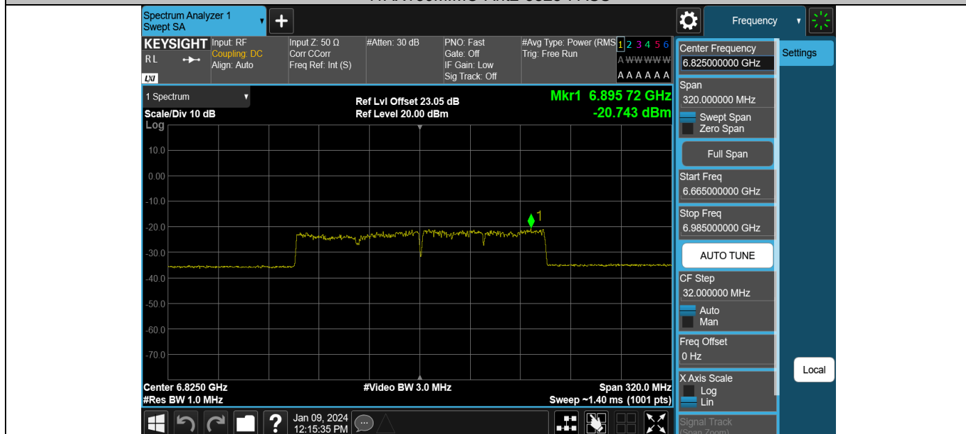
11AX160MIMO-Ant1-6985-PASS
