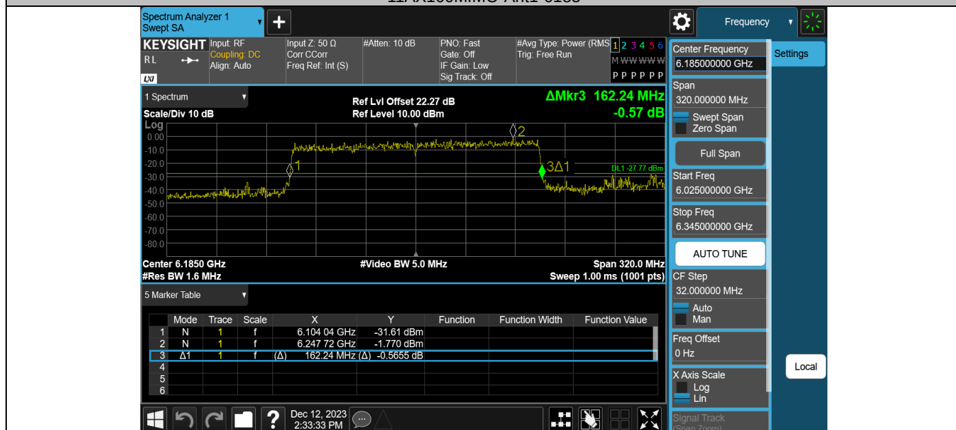
11AX160MIMO-Ant2-6185
