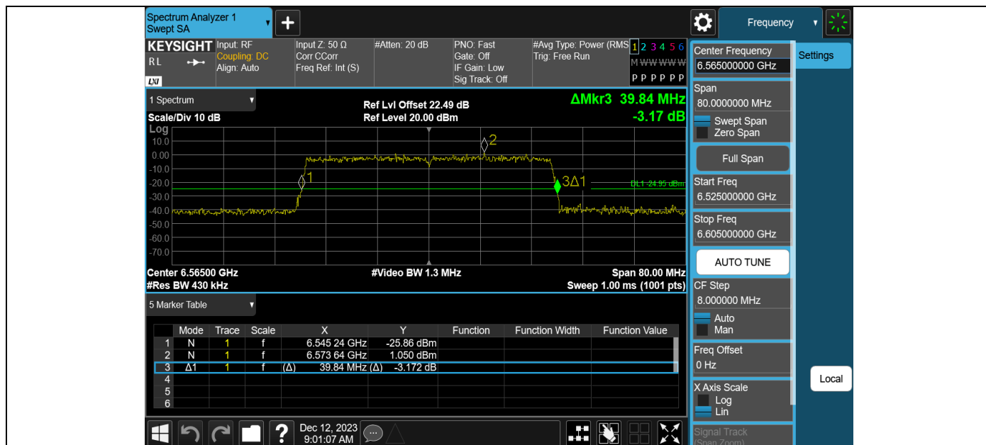
11AX40MIMO-Ant2-6565
