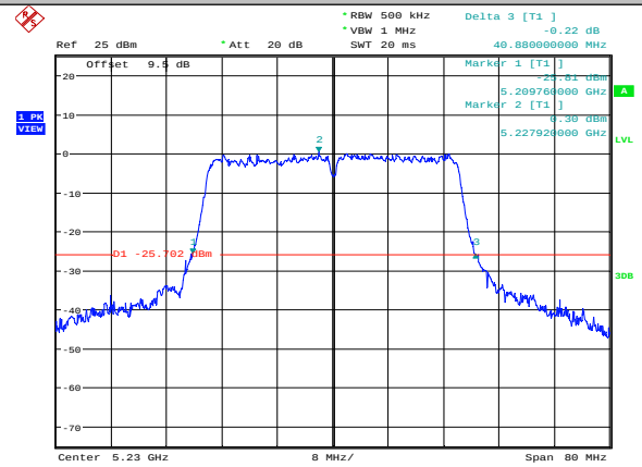
11AC40SISO-Ant2-5230
