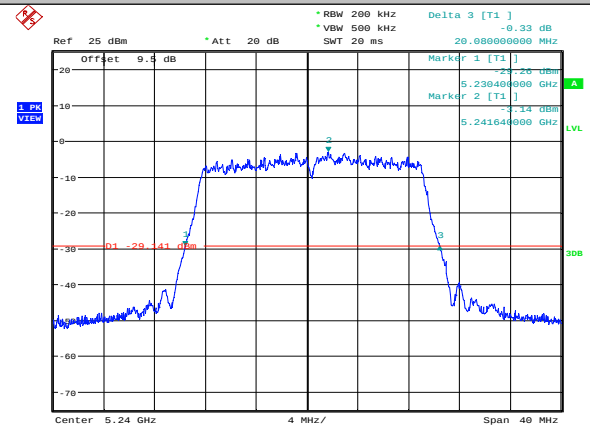
11AC20MIMO-Ant2-5240
