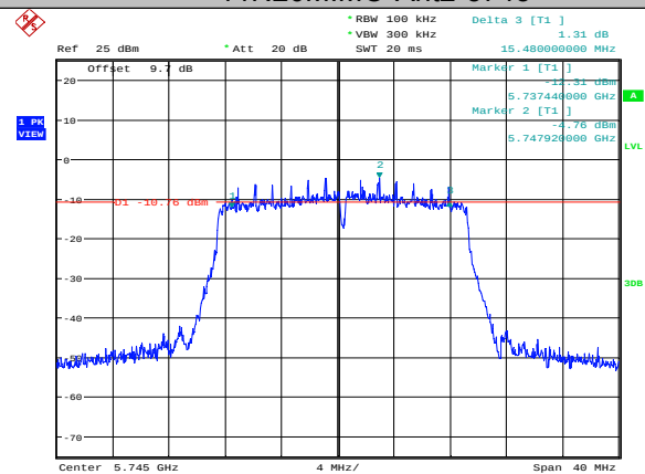
11N20MIMO-Ant2-5745
