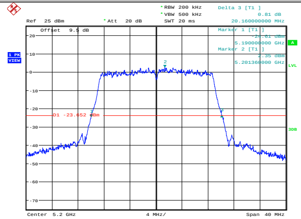
11AC20SISO-Ant2-5200
