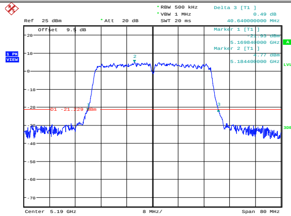
11N40SISO-Ant1-5190
