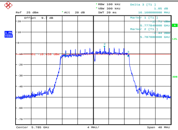
11N20MIMO-Ant2-5785
