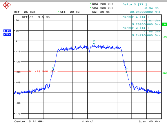
11AC20MIMO-Ant1-5240
