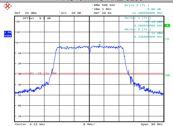
11AC40MIMO-Ant2-5230
