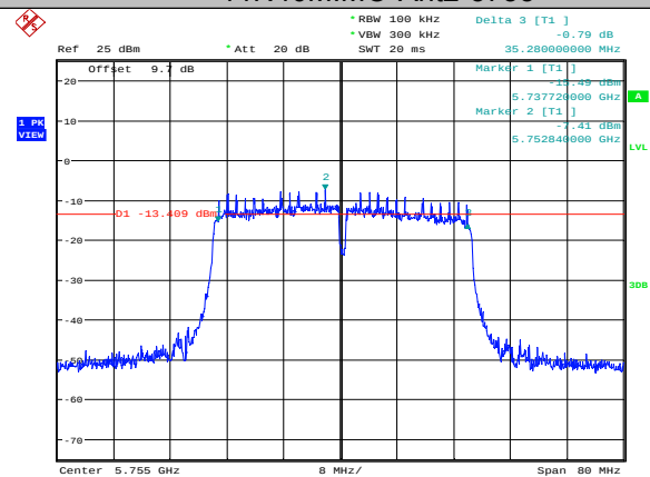
11N40MIMO-Ant2-5755
