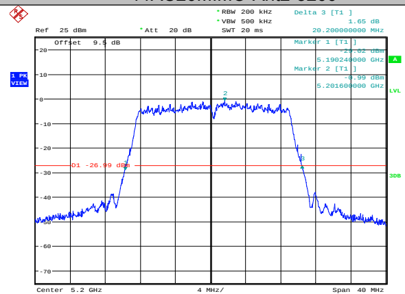
11AC20MIMO-Ant2-5200
