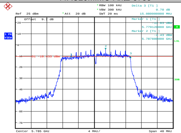
11AC20MIMO-Ant2-5785
