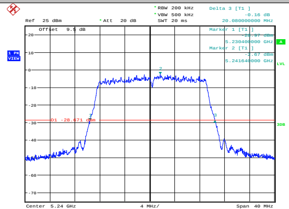
11N20MIMO-Ant2-5240
