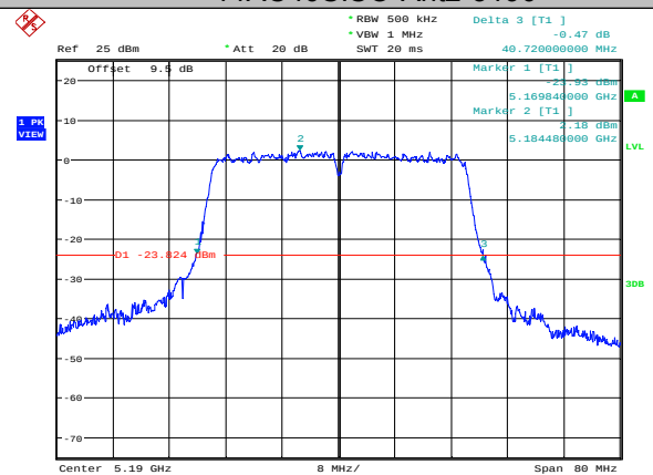
11AC40SISO-Ant2-5190
