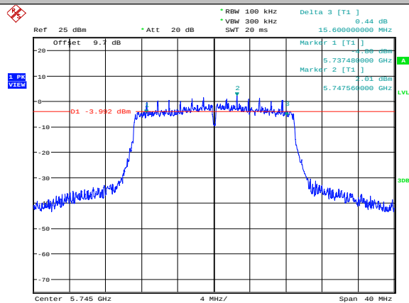
11AC20MIMO-Ant1-5745
