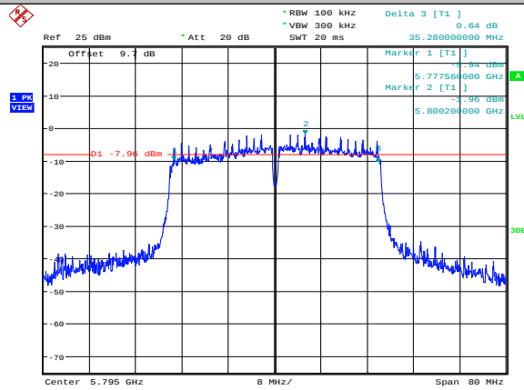
11AC40SISO-Ant1-5795
