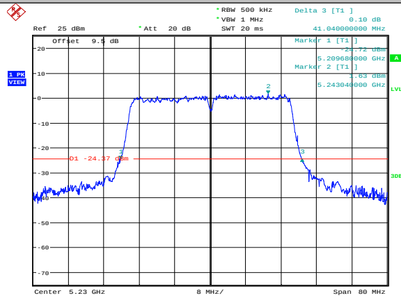
11AC40SISO-Ant1-5230
