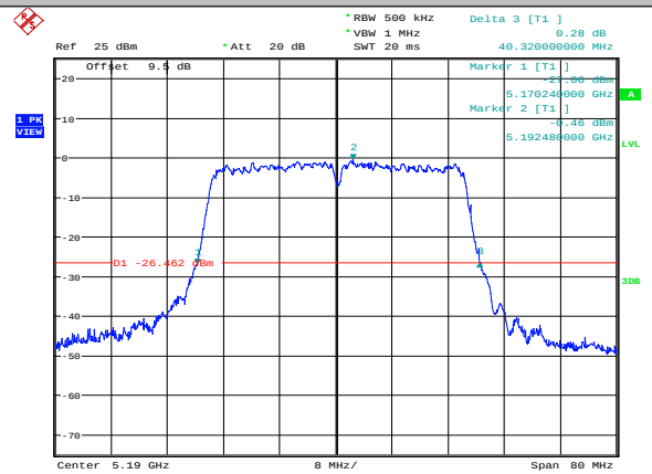
11AC40MIMO-Ant2-5190
