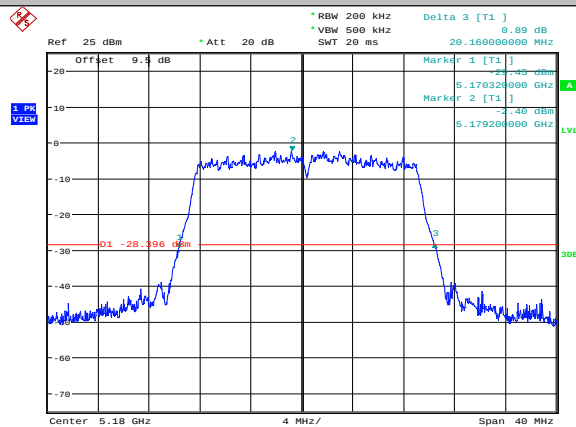
11AC20MIMO-Ant1-5180
