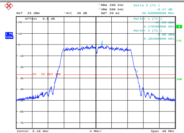
11AC20MIMO-Ant2-5180
