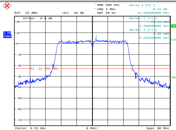
11N40SISO-Ant1-5230
