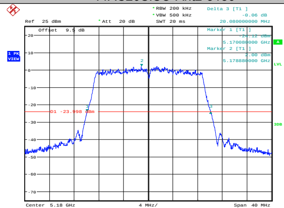
11AC20SISO-Ant2-5180
