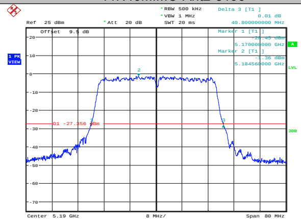
11N40MIMO-Ant2-5190
