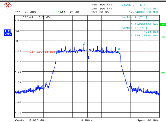
11N20MIMO-Ant2-5825
