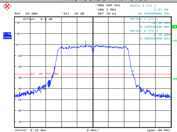
11AC40SISO-Ant1-5190
