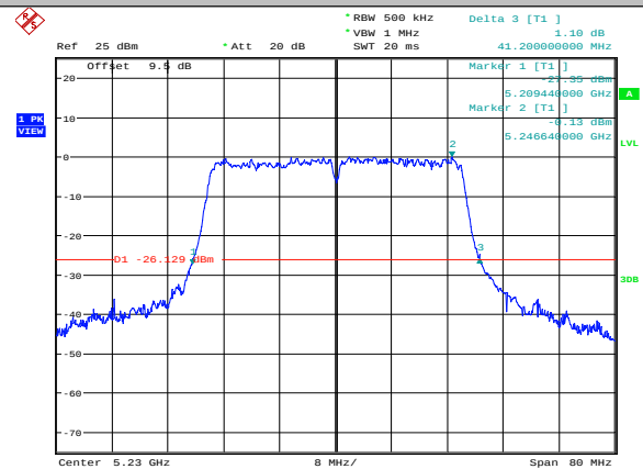
11N40SISO-Ant2-5230
