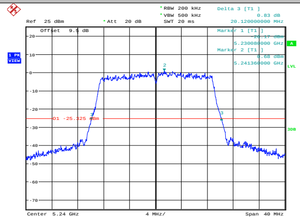
11AC20SISO-Ant2-5240
