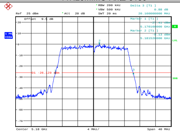
11N20MIMO-Ant2-5180
