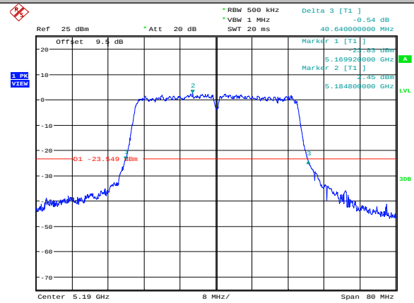
11N40SISO-Ant2-5190
