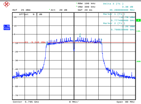
11AC40SISO-Ant2-5795
