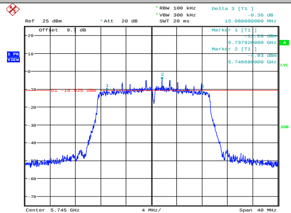
11AC20MIMO-Ant2-5745
