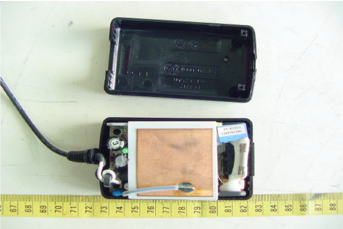
47. Internal View of Adaptor II
