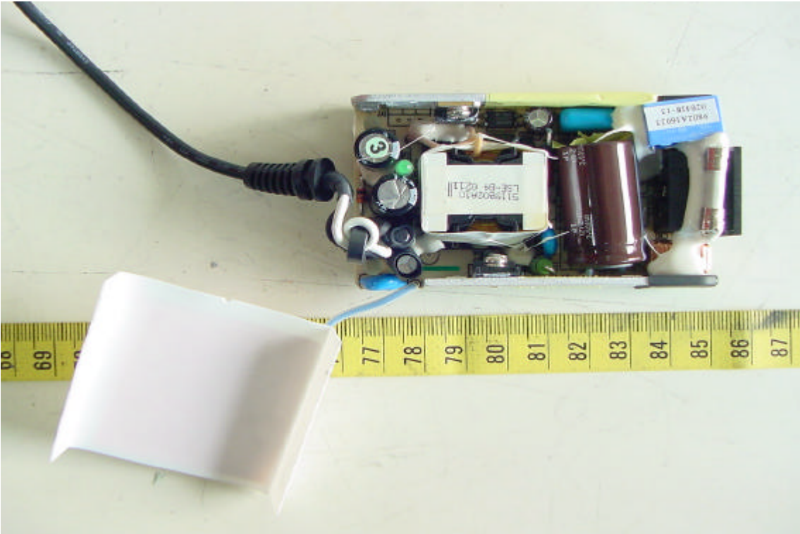
48. Component View of Adaptor PCB
