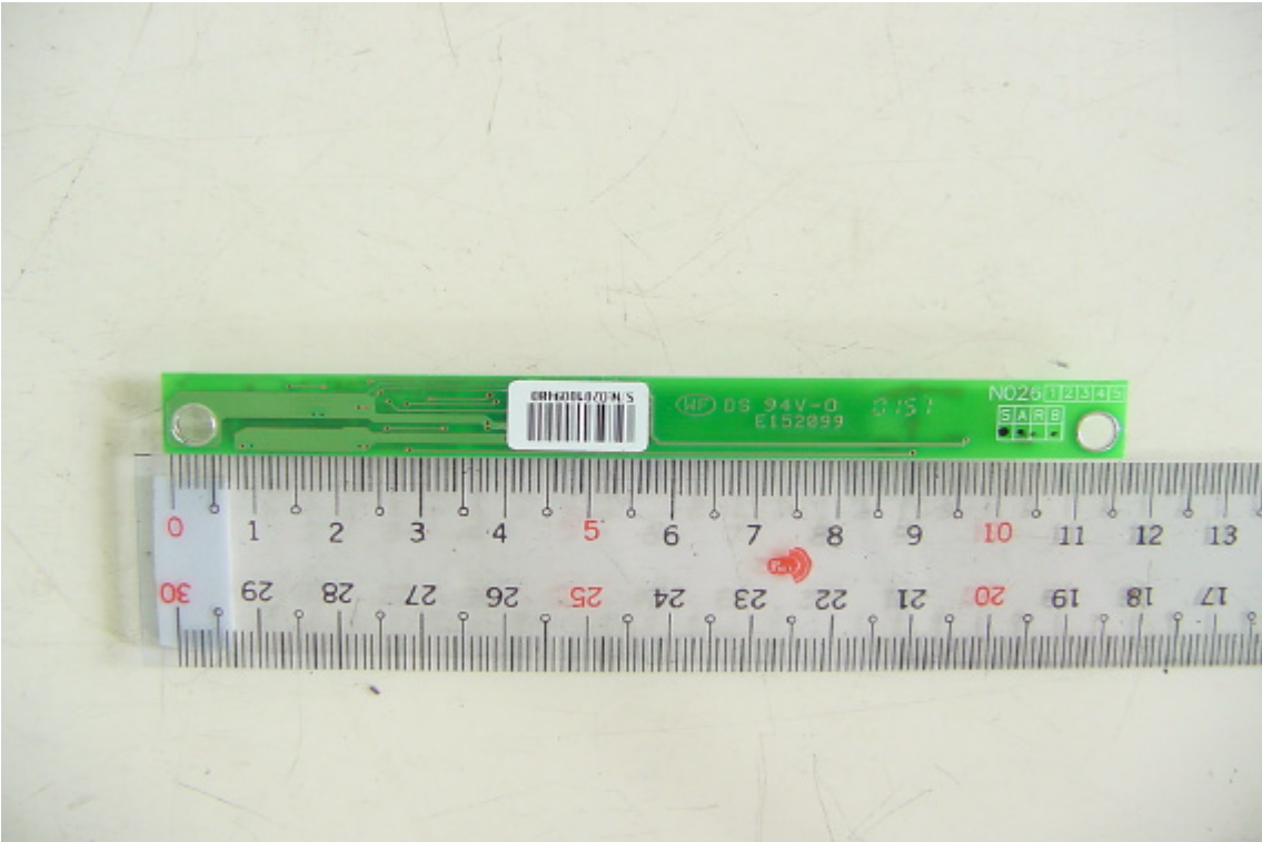
Solder View of PCB 8
