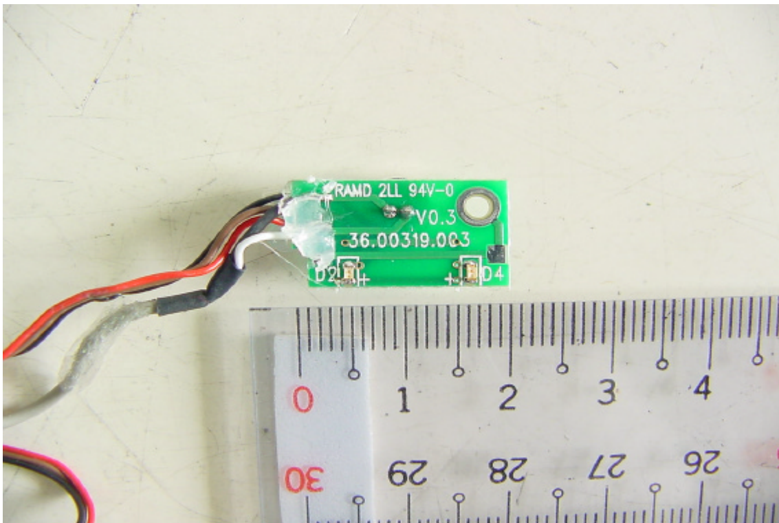
Solder View of PCB 9
