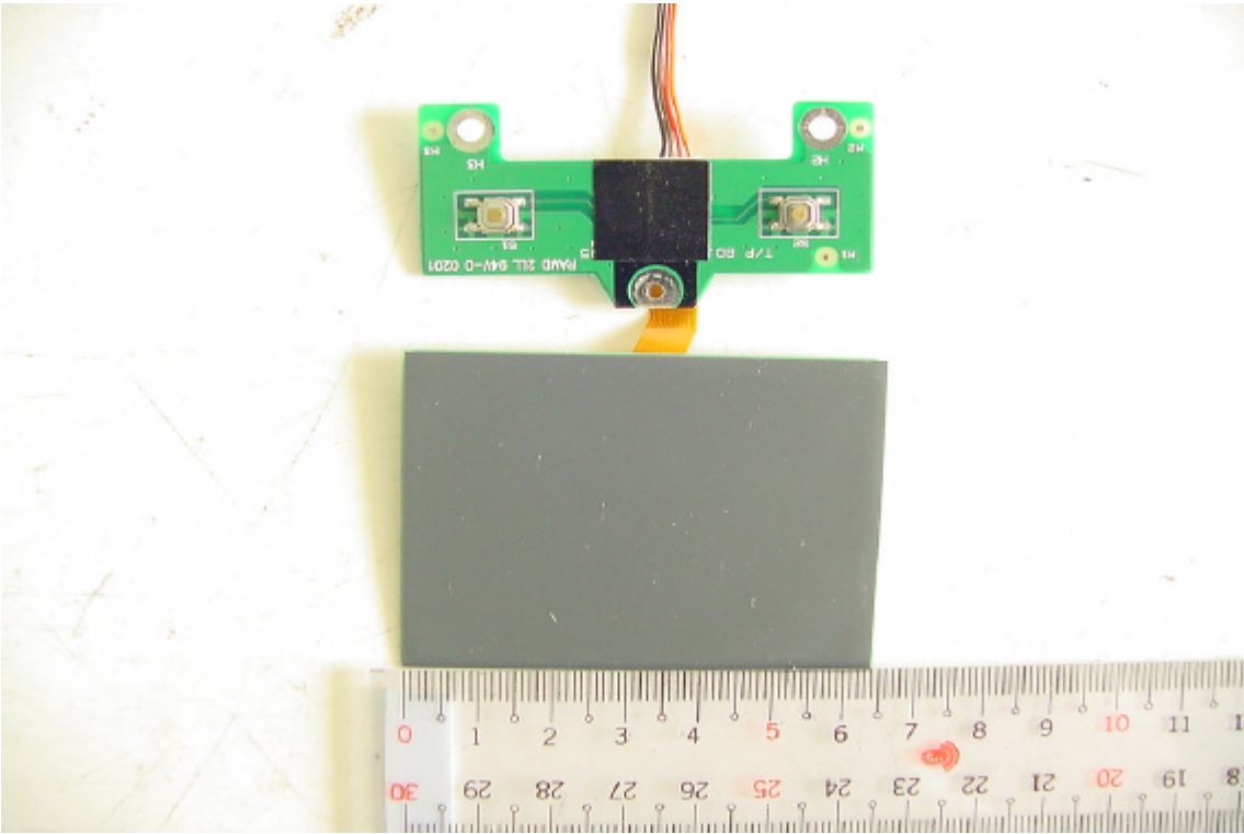
Solder View of Touch Panel's PCB
