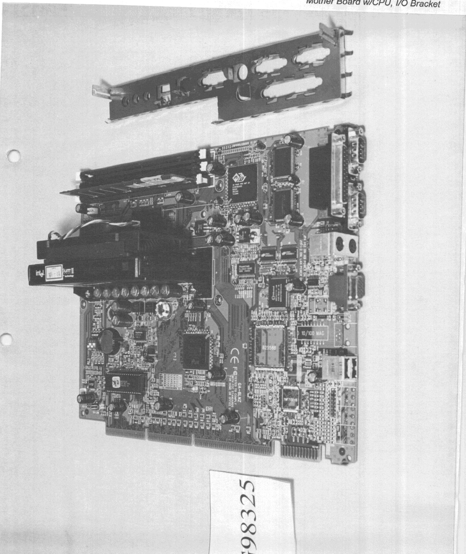
Figure 6 Mother Board w/CPU, I/O Bracket
