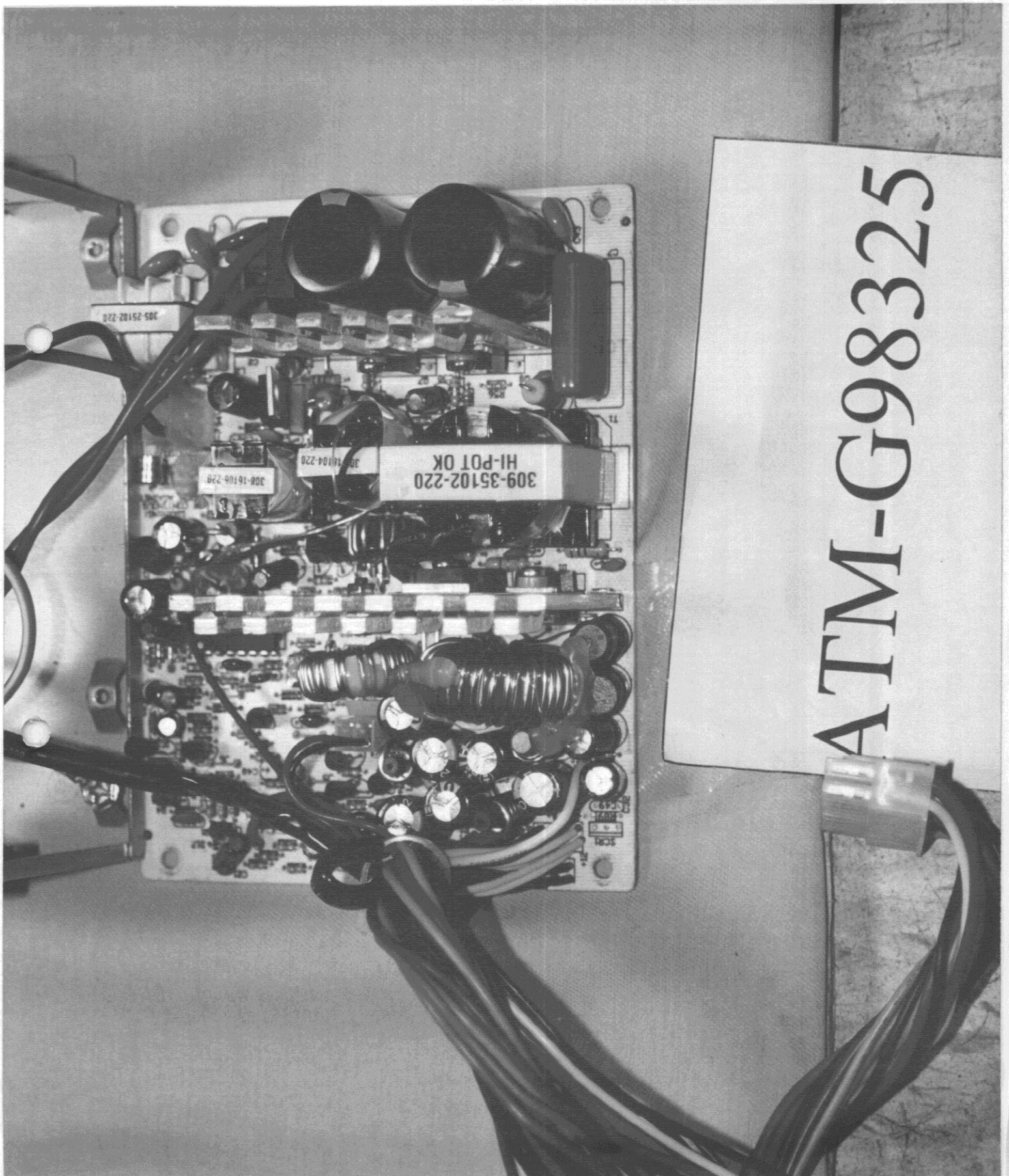
Figure 18 Switching Power Supply (PCB View)
