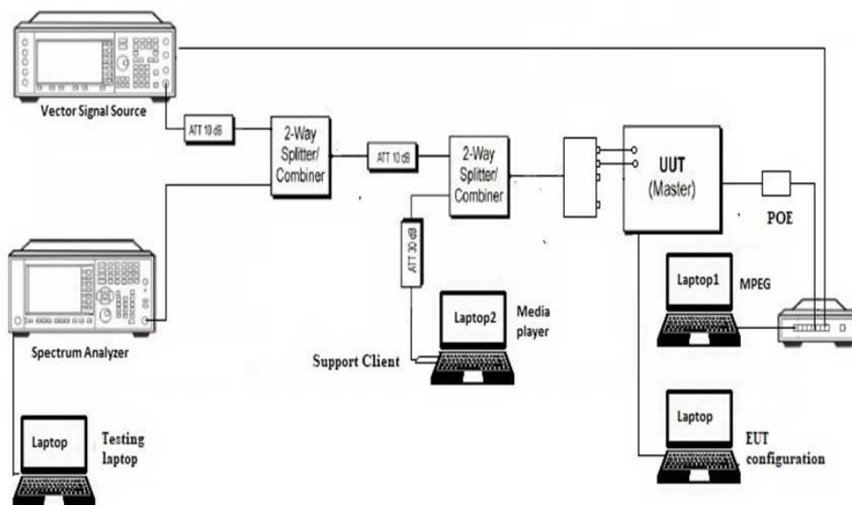
Setup for Master with injection at the Master
