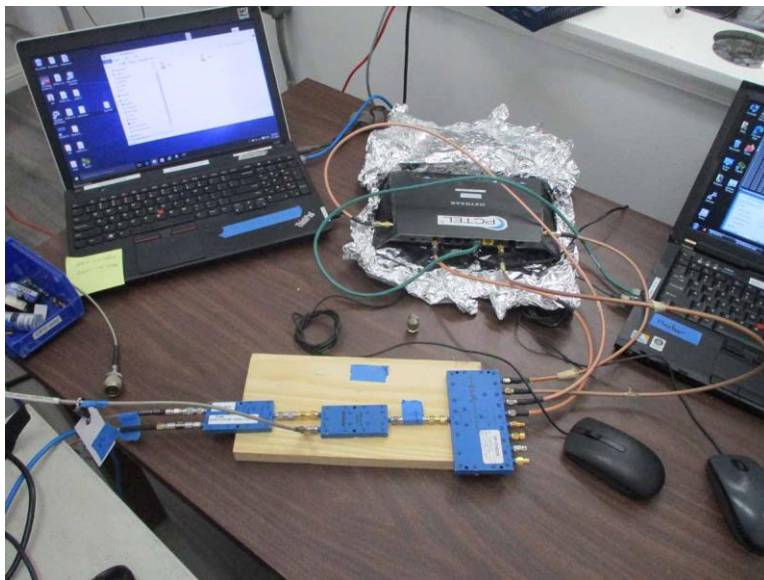
Test Setup, Client 1
