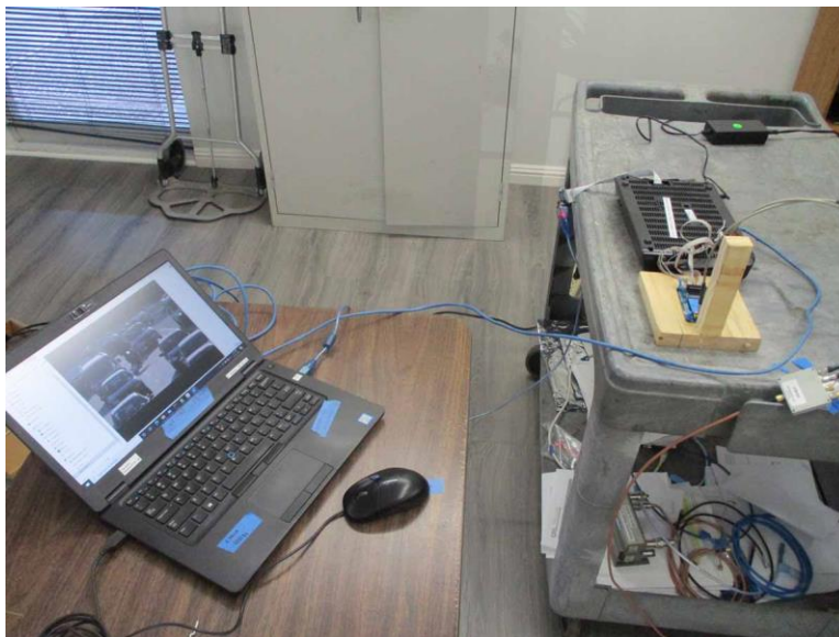
Test Setup, Client 5
