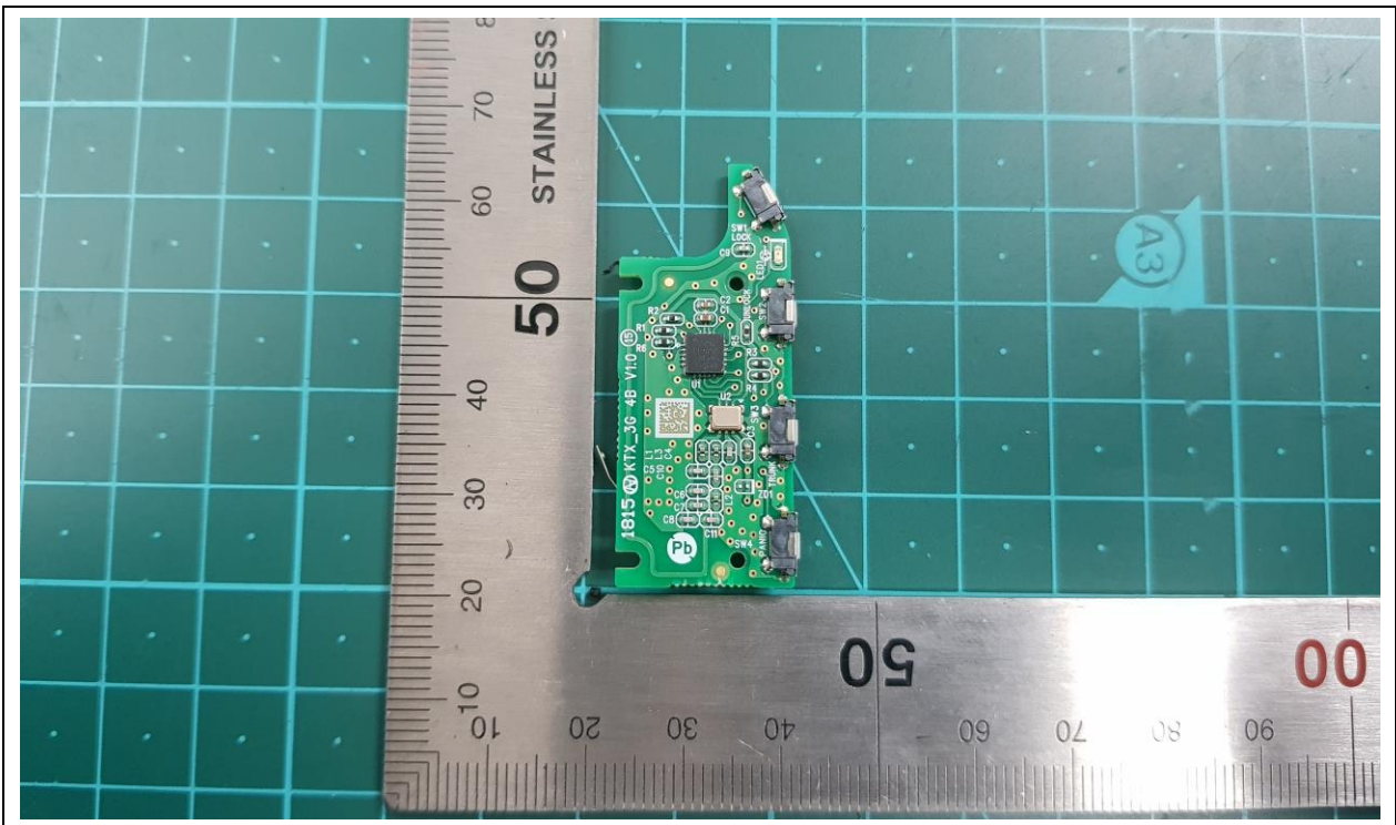
PCB Rear
