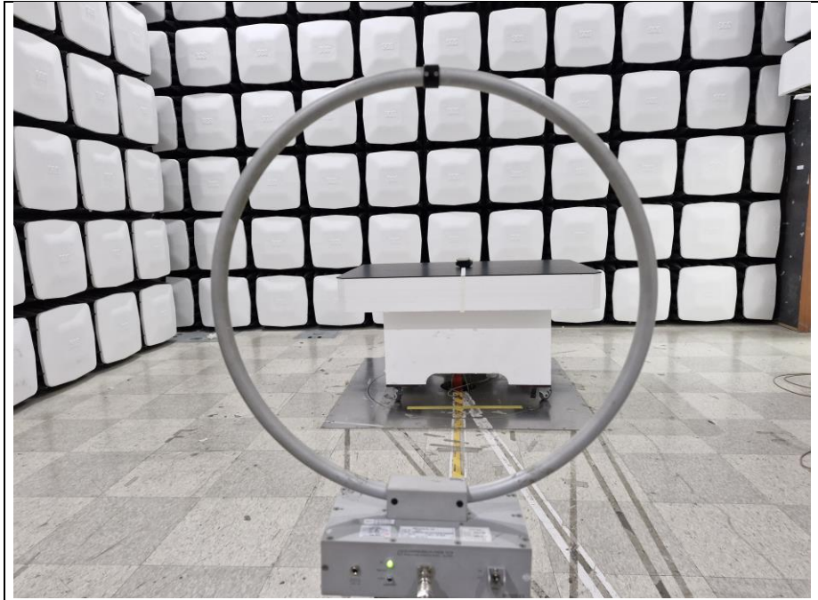
Photo of Test Set up (9 kHz ~ 30 MHz)
