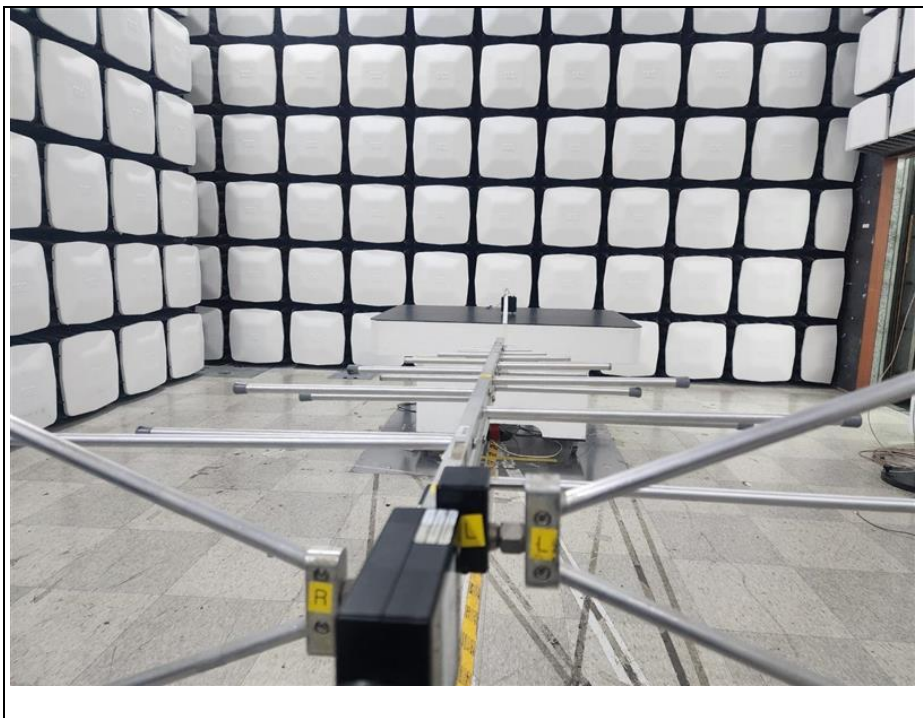
Photo of Test Set up (30 MHz ~ 1 GHz)
