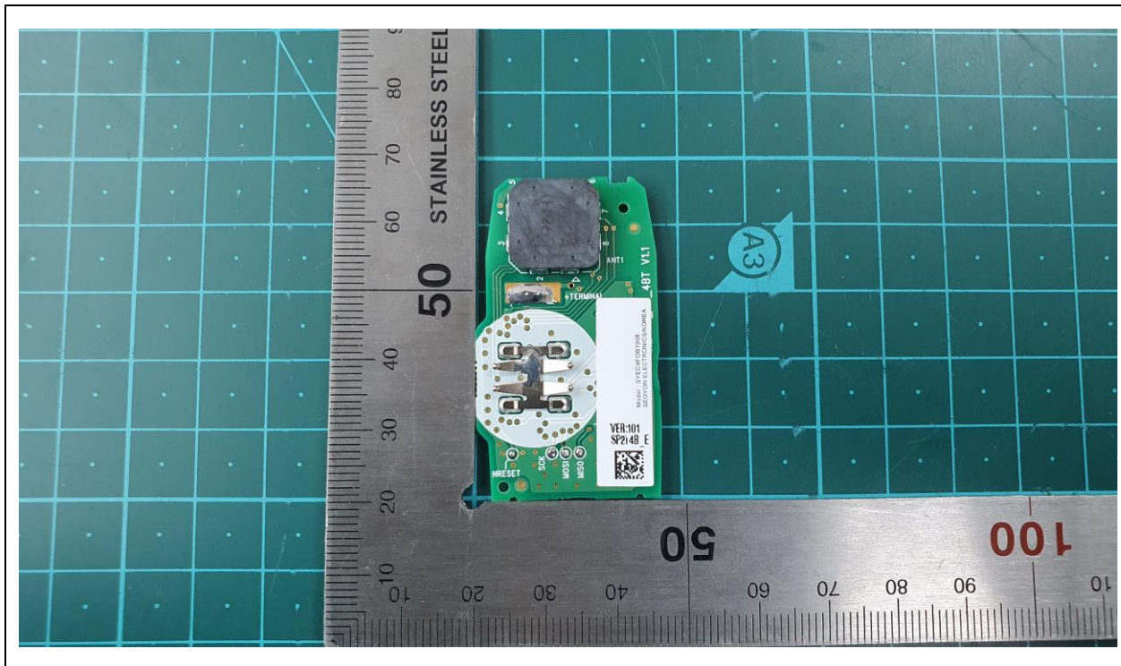
PCB Rear
