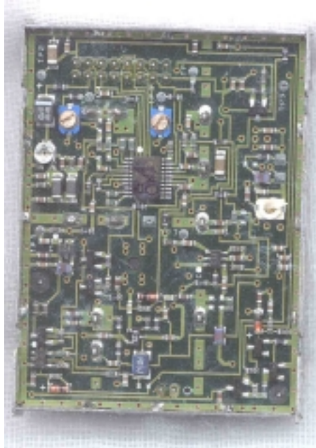
Photo 15. EUT, Bottom View of Transceiver Board with Shield Removed
