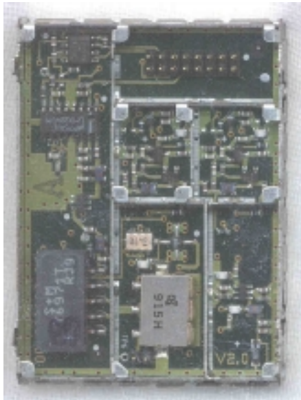
Photo 15. EUT, Bottom View of Transceiver Board with Shield Removed
