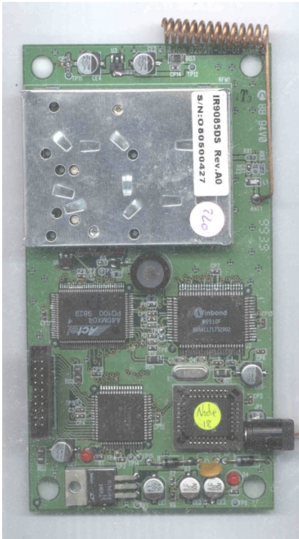
Photo 7. EUT, Bottom View of Main Board
