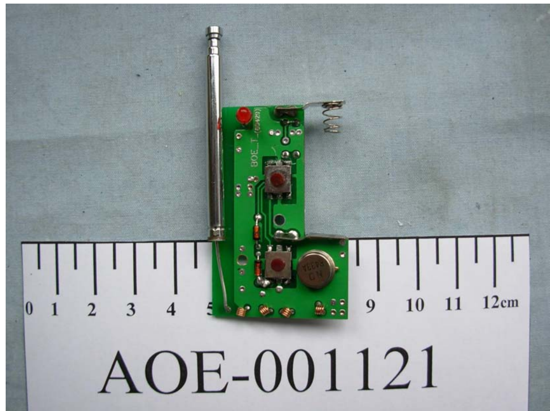
FIGURE 2 REMOTE RAIN (M/N: 5917) MAIN BOARD (COMPONENT SIDE)
