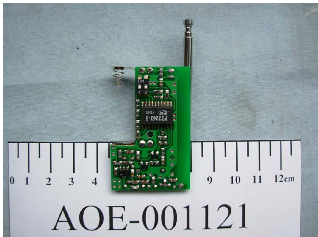
FIGURE 3 REMOTE RAIN (M/N: 5917) MAIN BOARD (SOLDERED SIDE)
