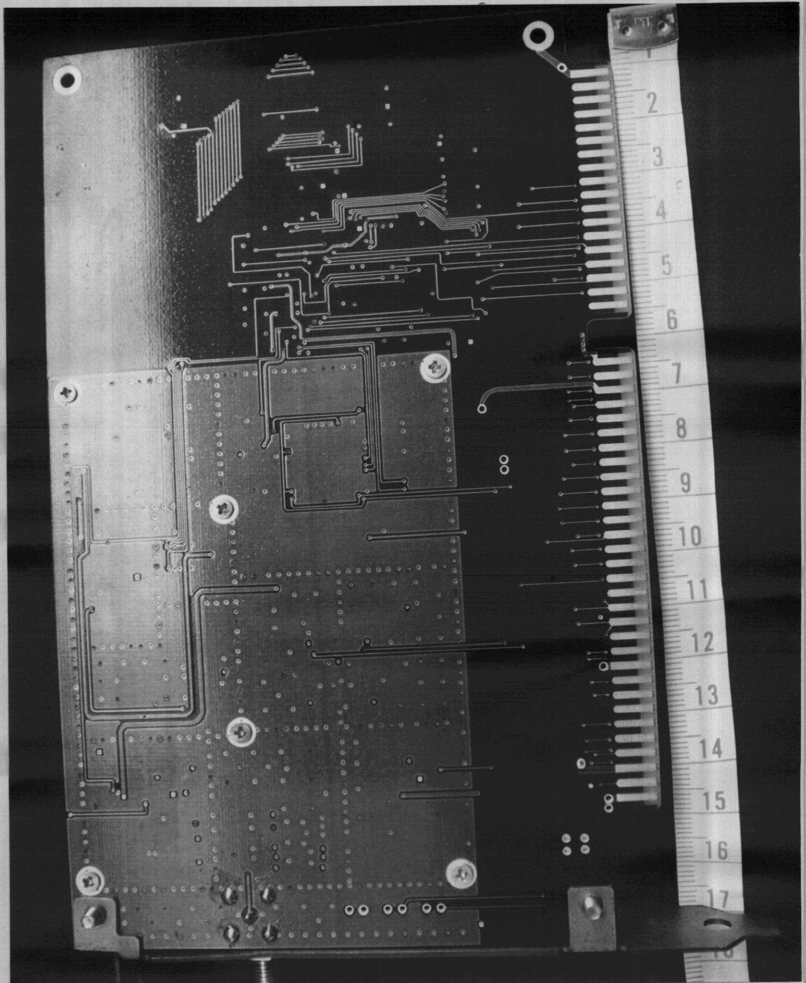
Solder View of PCB
