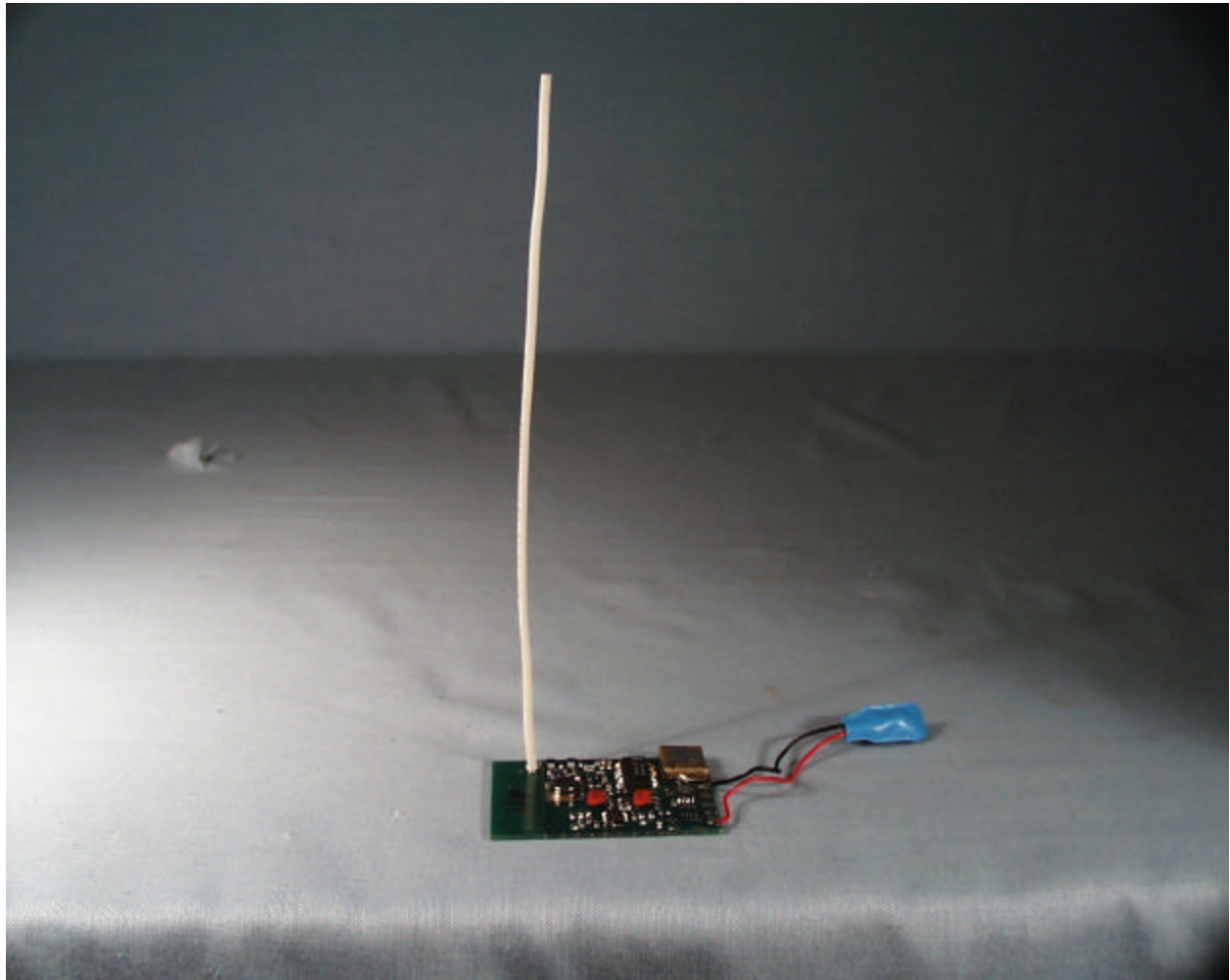
External view of the RA3R
