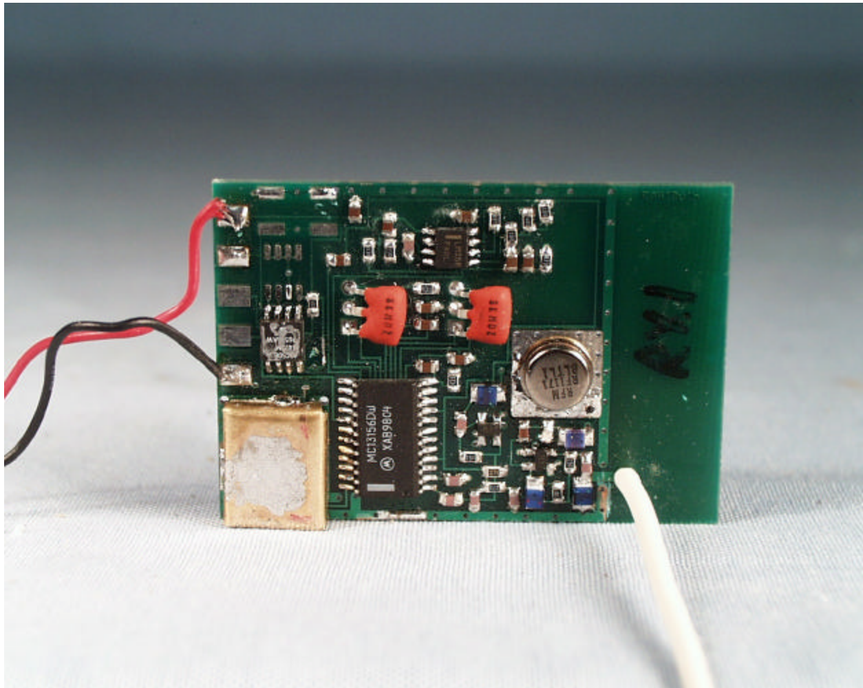
Component Side (with RF cans installed)
