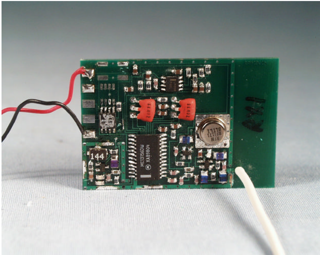
Component Side (with RF cans removed)
