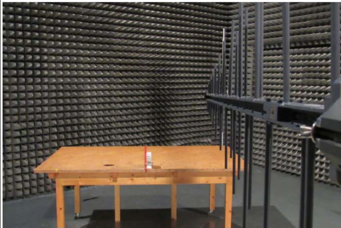
Setup radiated
