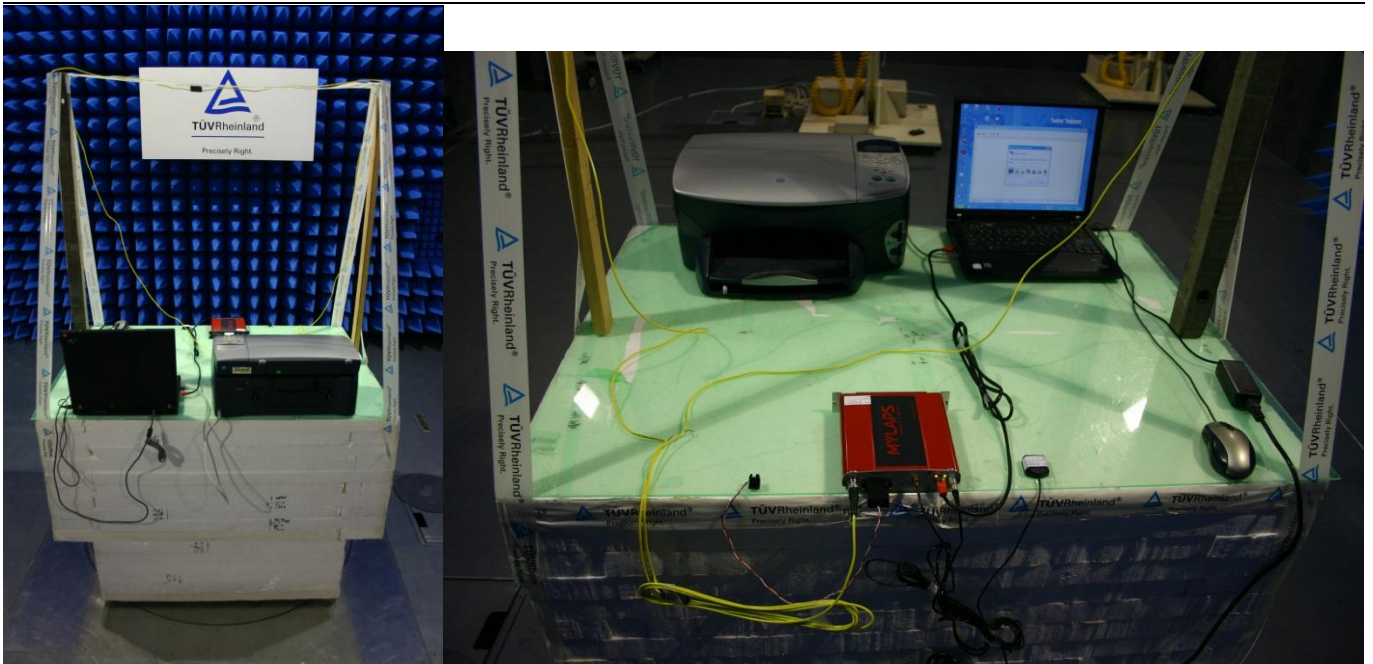
Testsetup photographs
