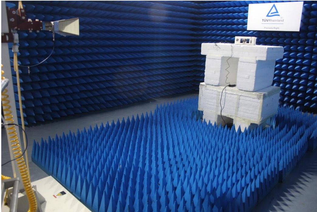
Test setup 1 – 18 GHz
