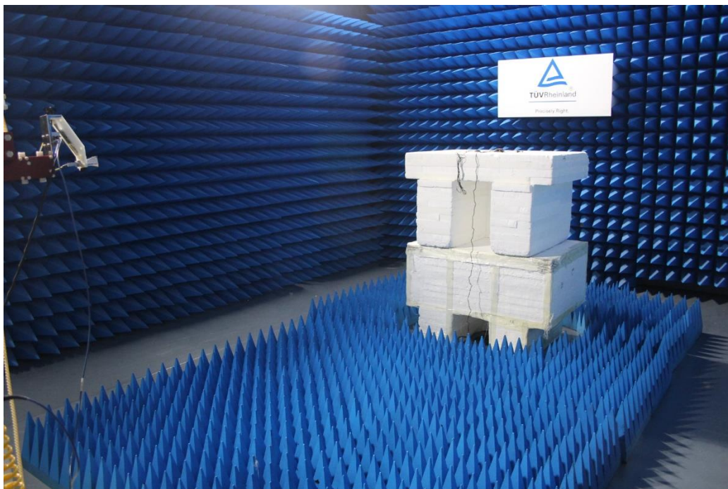
Test Setup 18 – 25 GHz
