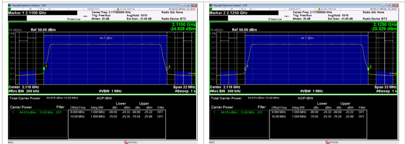
15 MHz Channel, 64 QAM
