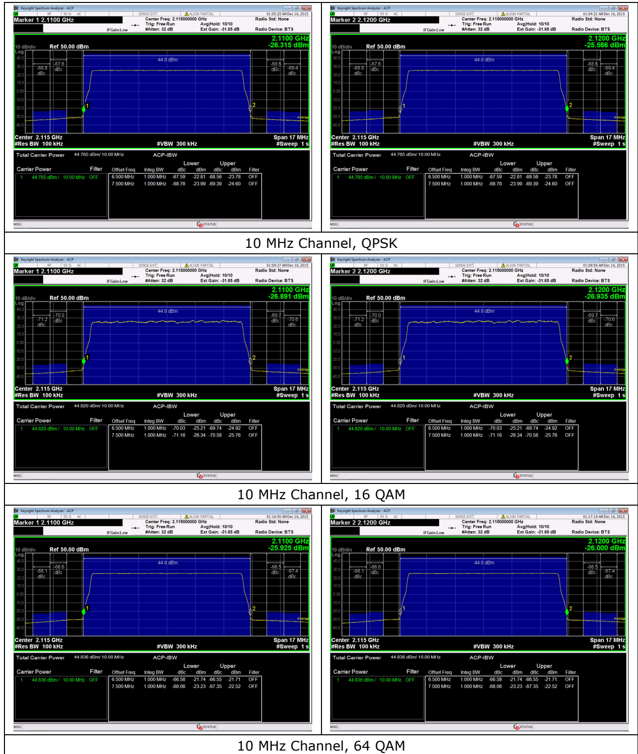
Figure 2: Transmit Power and band edge plots; 10 MHz channel
