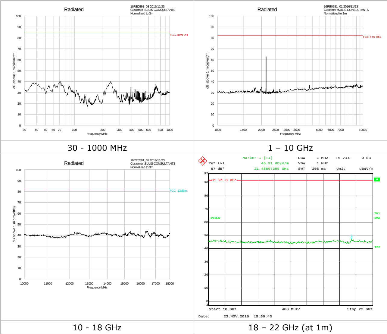
Figure 11: RSE pre-scans, 10 MHz channel
