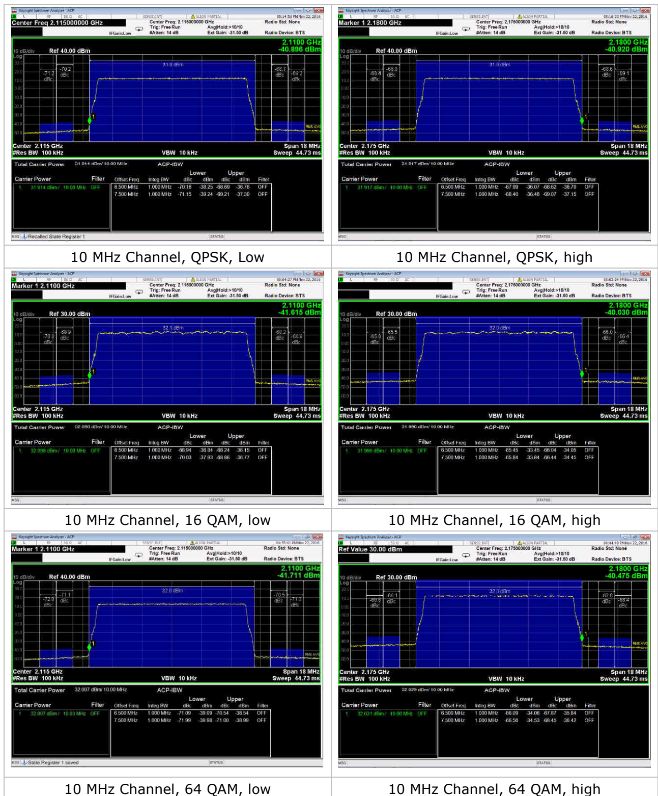
Figure 7: Band-edge emissions for 10 MHz channels
