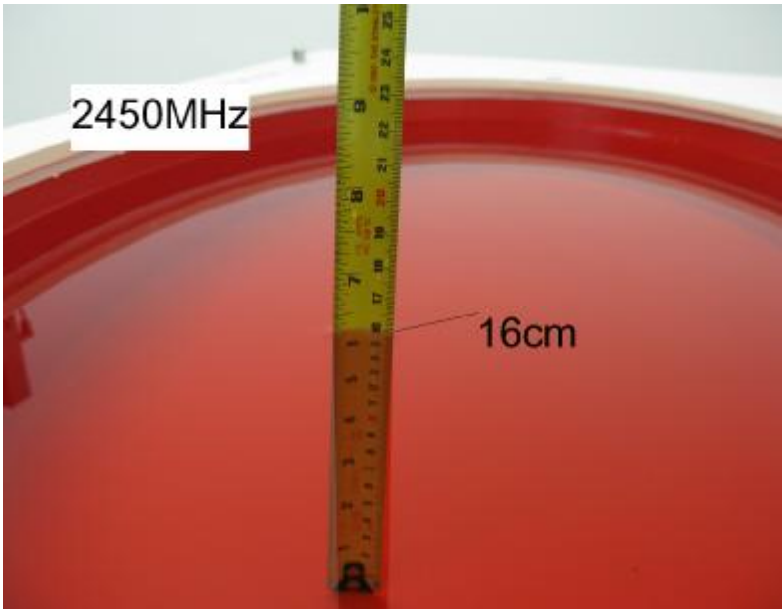
Fig.A-2 Photograph of the Body Tissue Simulant Liquid depth 15cm for Body Worn
