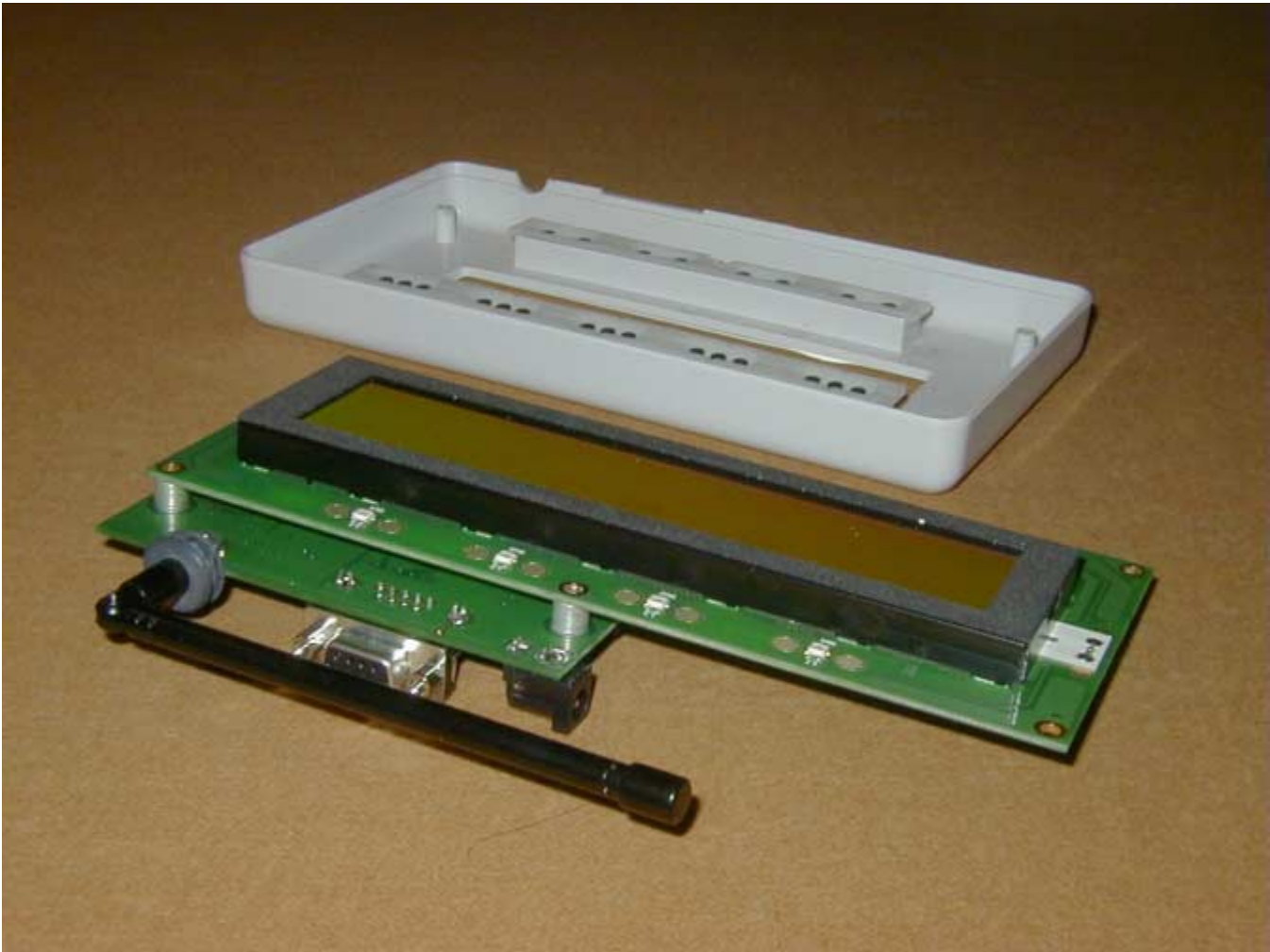
CONSOLE BOARD TOP
