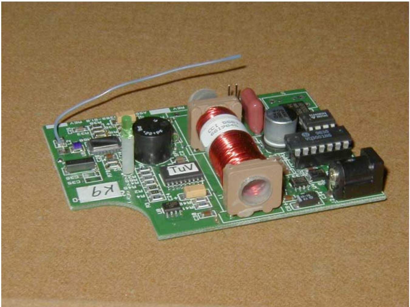
INDOOR ZONE BOARD
