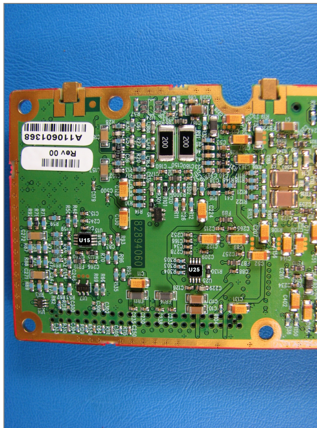
Photo 12 : MDM Board – Bottom Left
