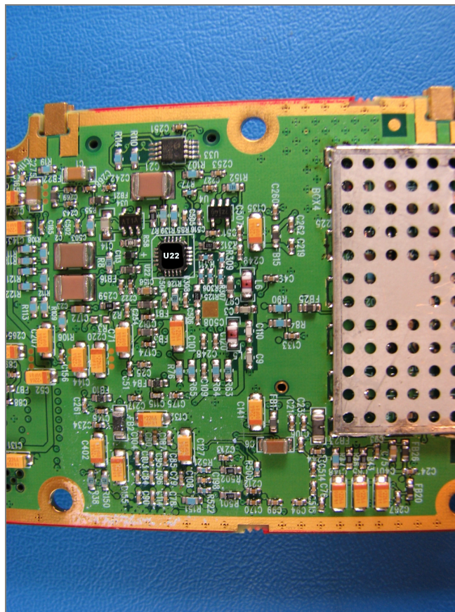
Photo 13 : MDM Board – Bottom Right
