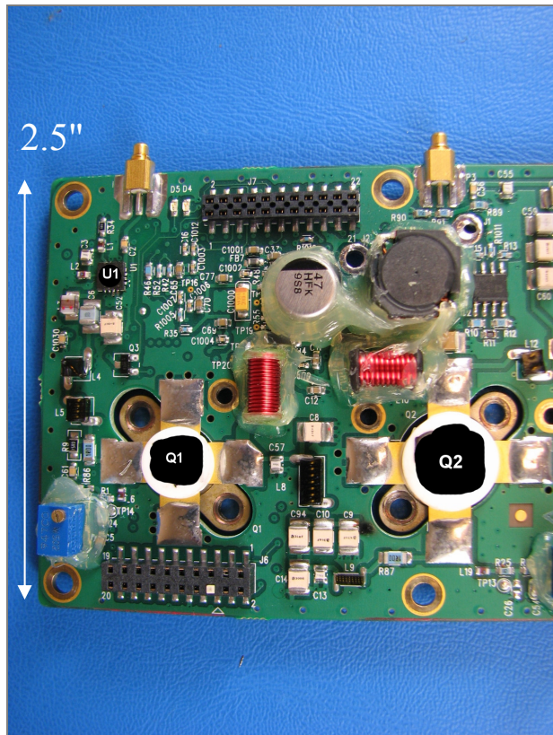
Photo 14 : TX Board – Top Left
