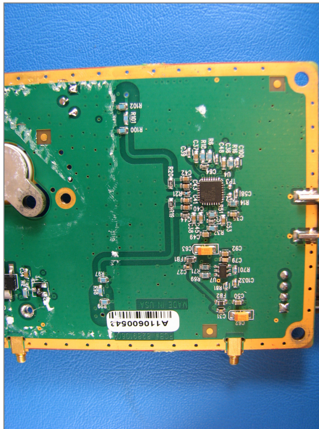
Photo 17 : TX Board – Bottom Right
