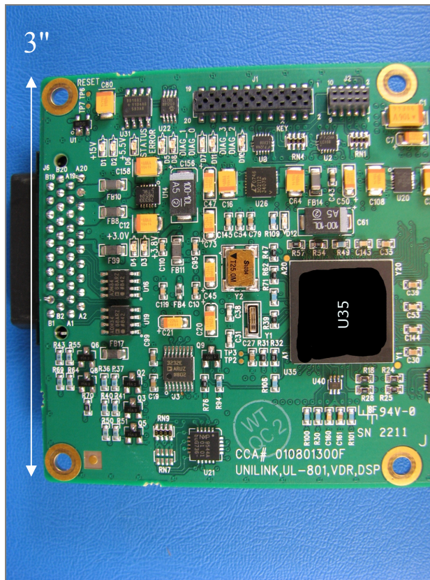
Photo 6 : DSP Board – Top Left
