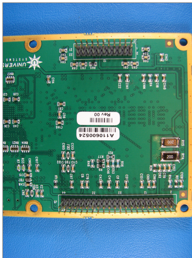
Photo 9 : DSP Board – Bottom Right
