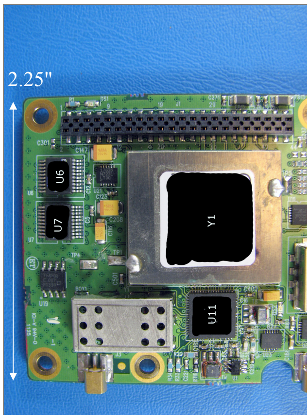
Photo 10 : MDM Board – Top Left
