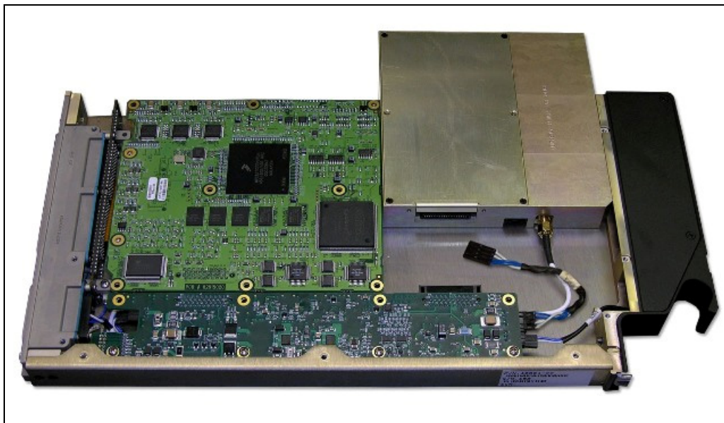
Photo 2 : UL-801 with VDR Module Disconnected from Power Supply
