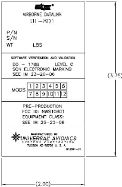
Figure 2 : UL-801 ID Label
