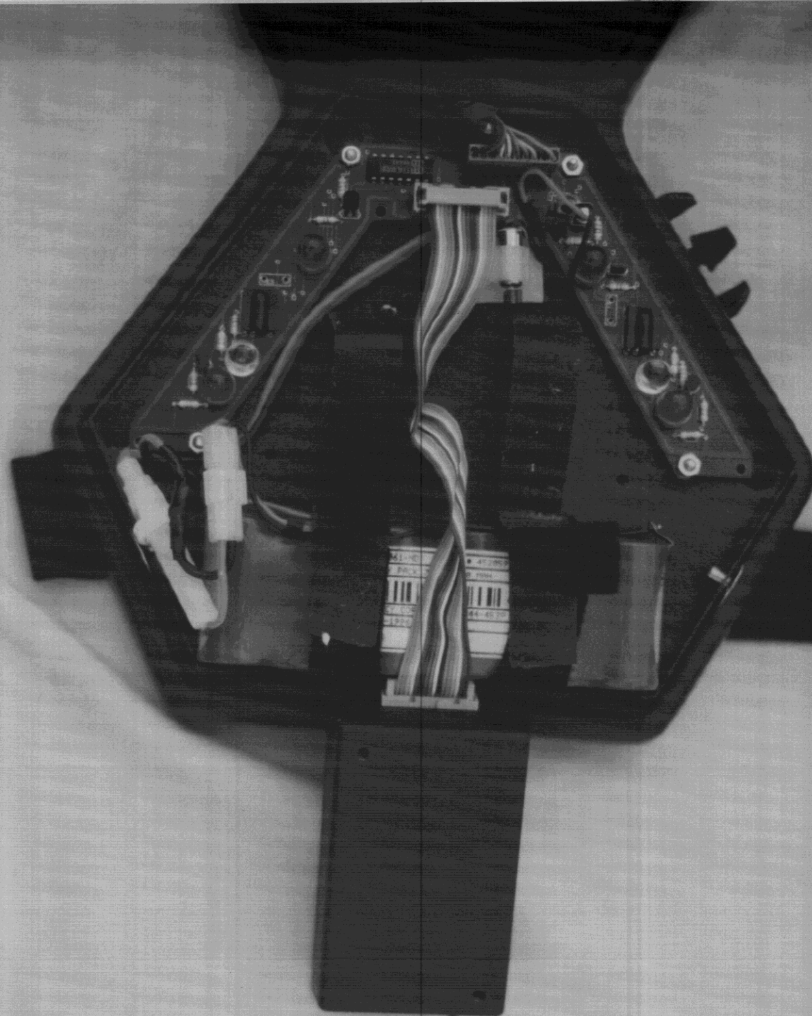
FRONT ELECTRONICS ENCLOSURE SIDE WITH COVER OFF AND RF MODULE UNMOUNTED FCC ID: NWQSC98V1
