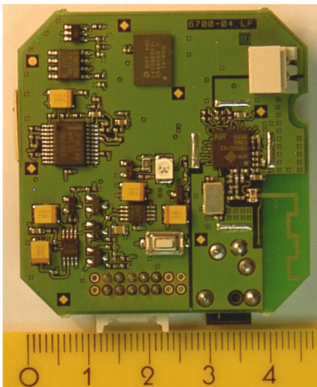
HELLO BIKER – FCC ID NWD BC6715 FRONT VIEW OF PCB – NOV. 2006
