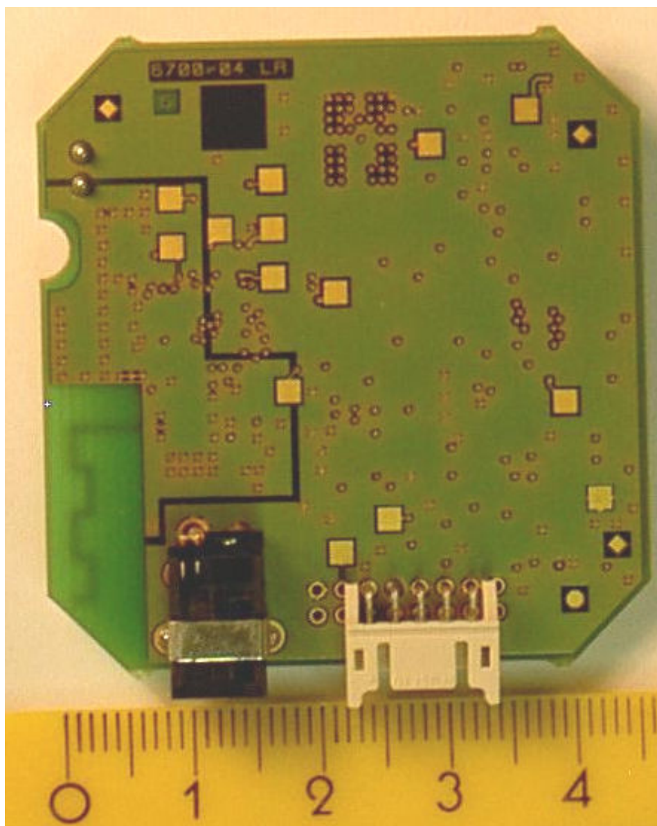
HELLO BIKER – FCC ID NWD BC6715 REAR VIEW OF PCB – NOV. 2006
