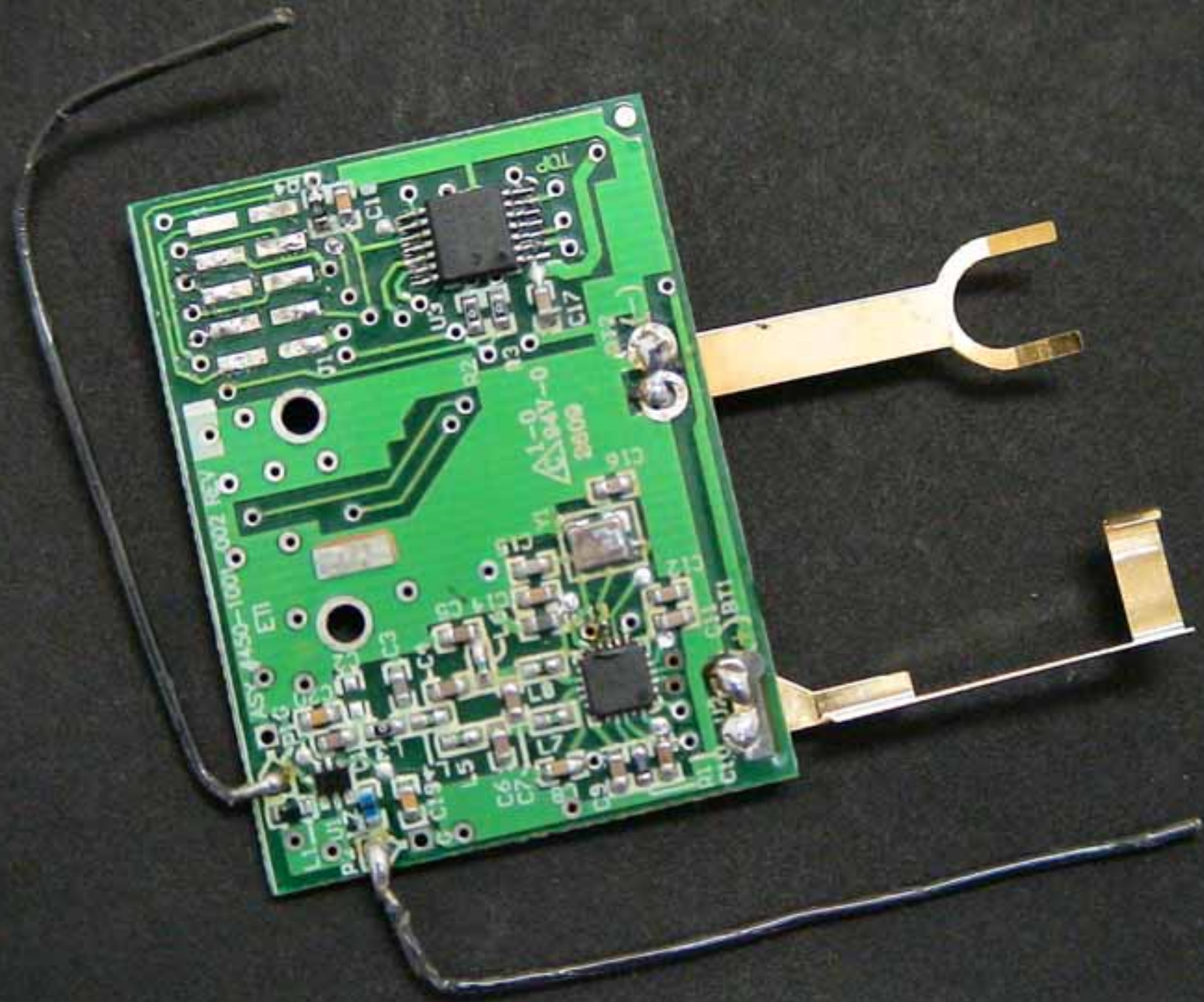
PCB (bottom)
