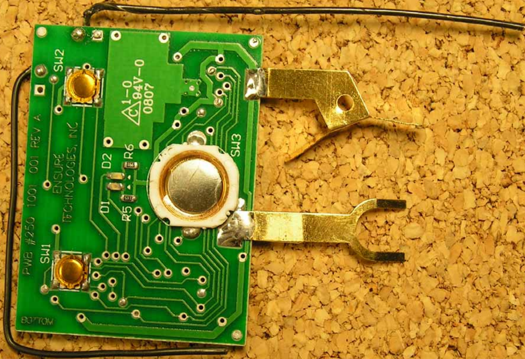
PCB (top) XC-3E (3 buttons populated)
