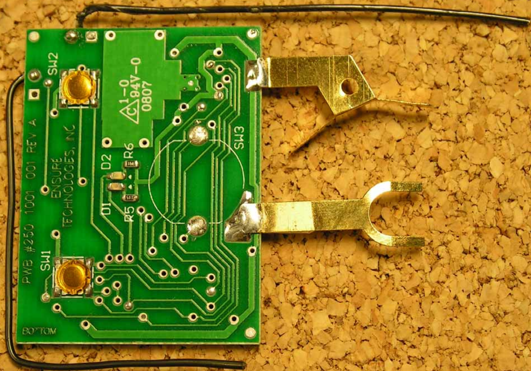
PCB (top) XC-3 (2 buttons populated)
